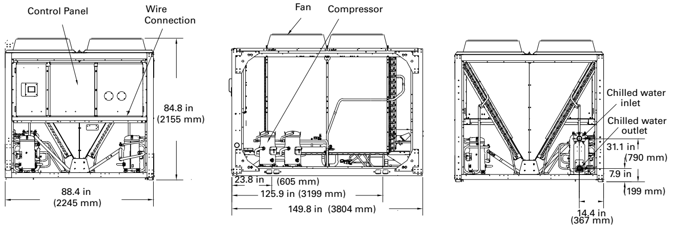
Figure 7. CGAM 52 ton (comprehensive acoustic package version), 60 and 70 ton (compact and comprehensive acoustic package versions), CXAM 46 (comprehensive acoustic package version), 52-70 ton (compact and comprehensive acoustic package versions)
