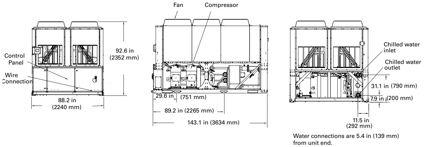
Figure 9. CGAM 80 and 90 (compact version)
