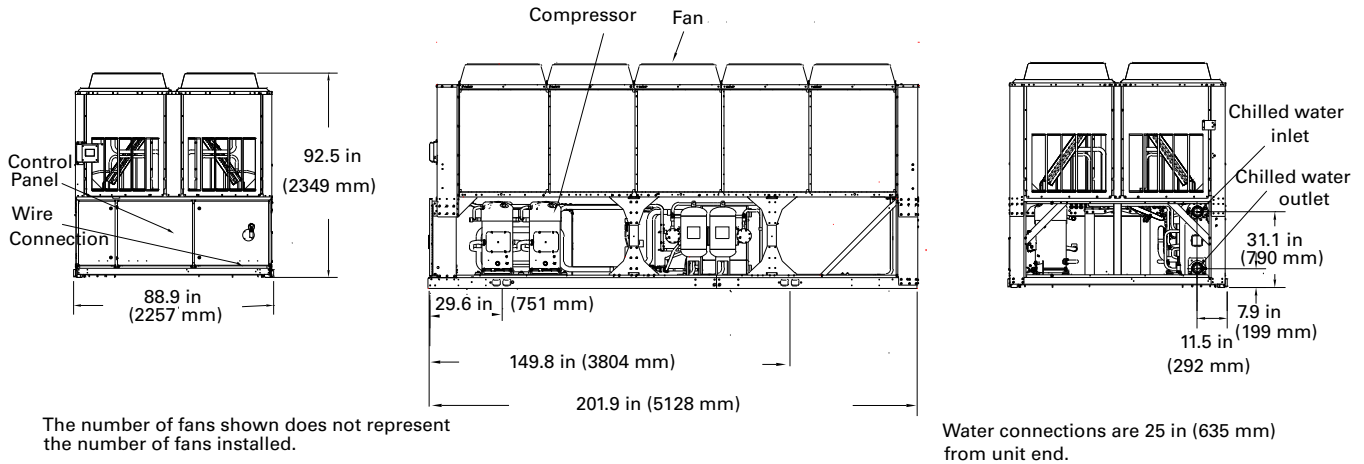
Figure 13. CGAM 110 and 120 (comprehensive acoustic package versions), 140 (compact version), CXAM 90 (comprehensive acoustic package versions), 100 (compact and comprehensive acoustic package versions), 110 and 120 (compact version)
