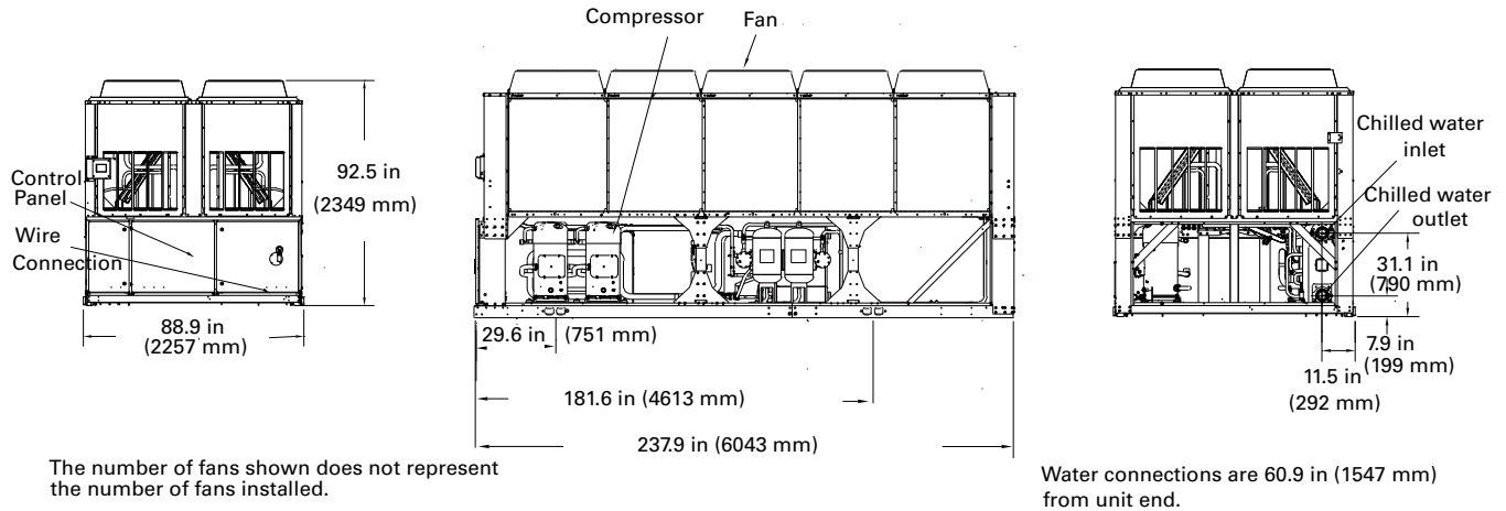
Figure 15. CGAM 140 (comprehensive acoustic package version), 150 and 160 (compact and comprehensive acoustic package versions), CXAM 110 and 120 (comprehensive acoustic package version), 140, 150 and 160 (compact)
