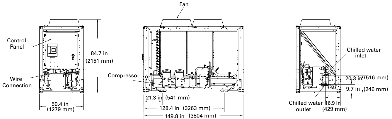
Figure 3. CGAM 26 ton (comprehensive acoustic package version), 30 and 35 ton (compact and comprehensive acoustic package versions), CXAM 23 ton (comprehensive acoustic package version), 26-35 ton (compact and comprehensive acoustic package versions)
