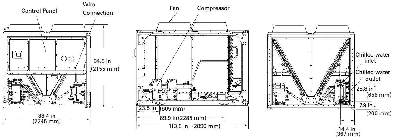
Figure 5. CGAM 40 and 46 ton (compact and comprehensive acoustic package versions), 52 ton (compact version), CXAM 40 (compact and comprehensive acoustic package versions), 46 ton (compact version)
