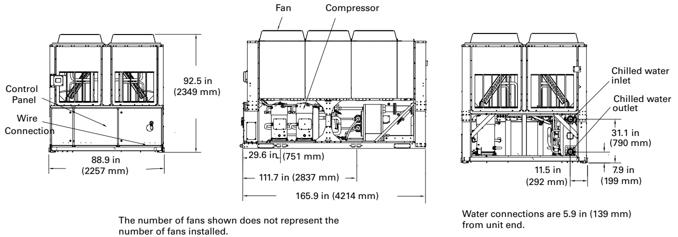
Figure 11. CGAM 80 and 90 (comprehensive acoustic package version), 100 (compact and comprehensive acoustic package versions), 110 (compact version), CXAM 80 (compact and comprehensive acoustic package versions), 90 (compact version)
