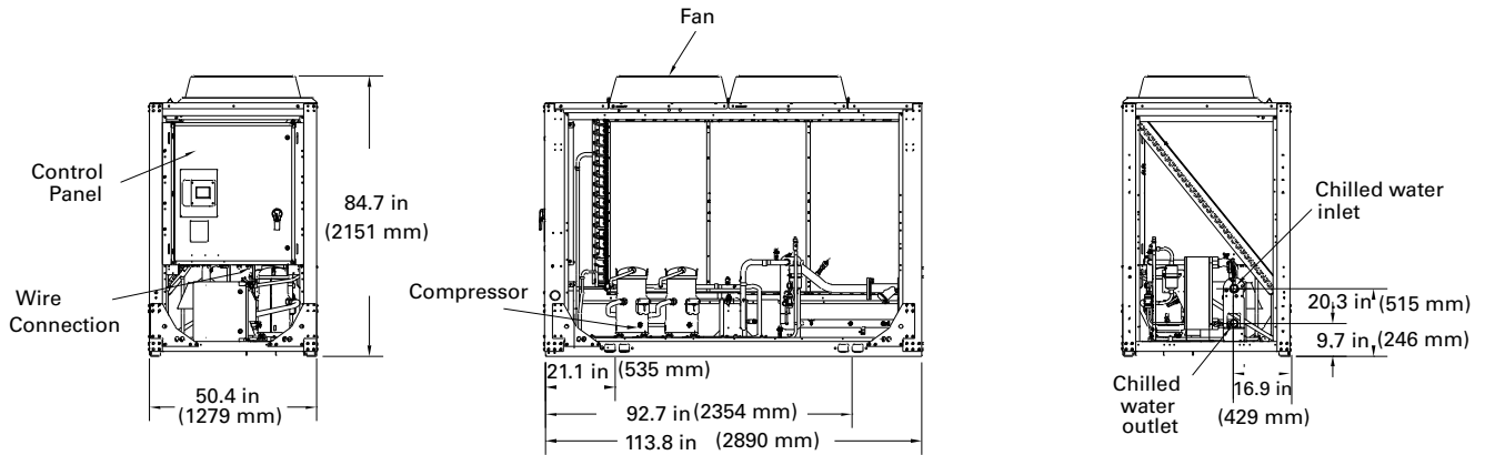
Figure 1. CGAM 20 and 23 ton (compact and comprehensive acoustic package versions), 26 ton (compact version), CXAM 20 (compact and comprehensive acoustic package version), 23 (compact version)
