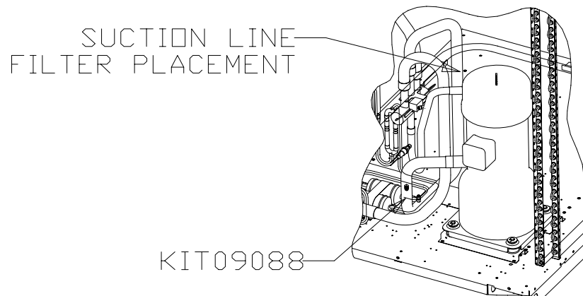
Figure 1. Compressor replacement illustration for TWA100AD**D, TWA120A3**D, TWA120A4**D, and TWA120AW**D
