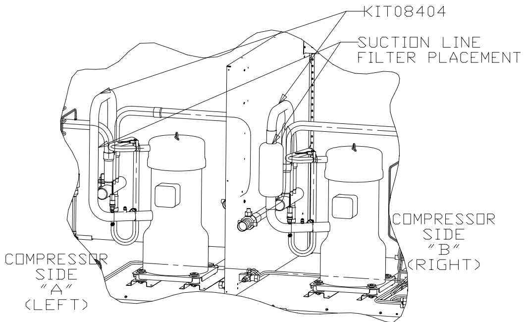
Compressor replacement illustration for TWA240B
