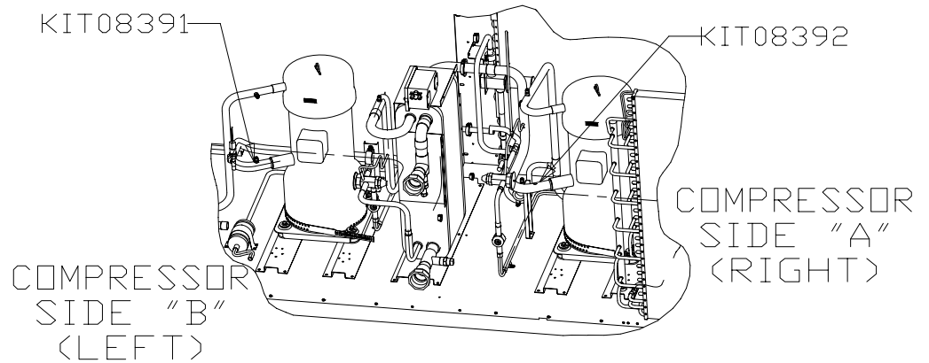
Compressor Replacement Illustration for CGA180B
