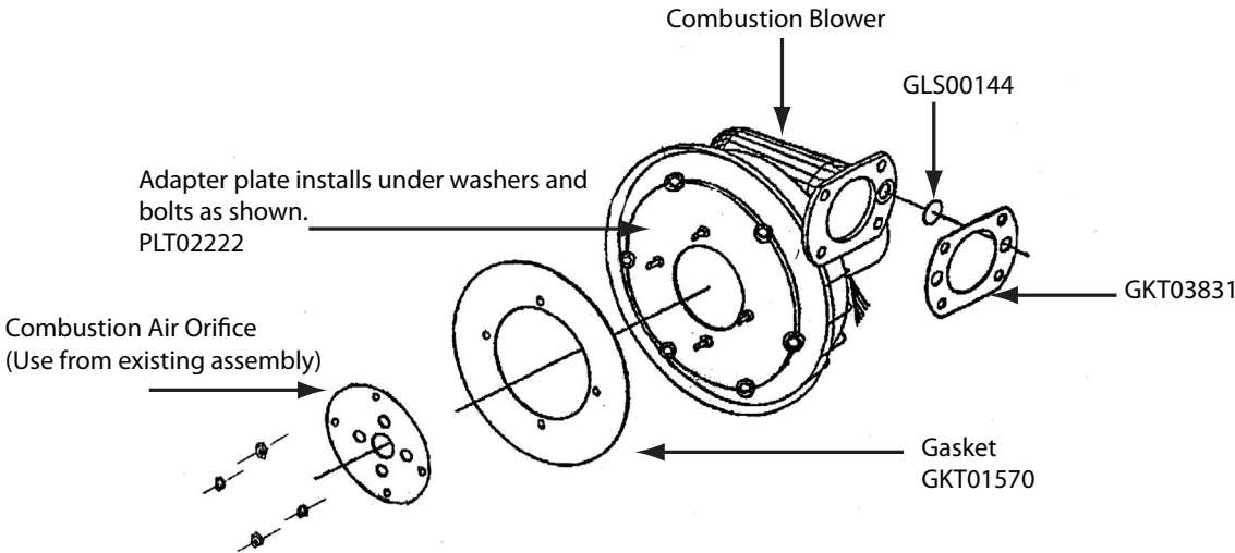
Figure 1. Combustion blower kit
