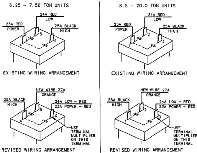
Figure 2. Combustion fan relay (CFR) wiring change
