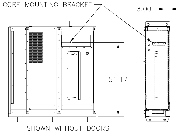
Figure 1. AFDE Unit-Mounted Drive (Frame 3)
