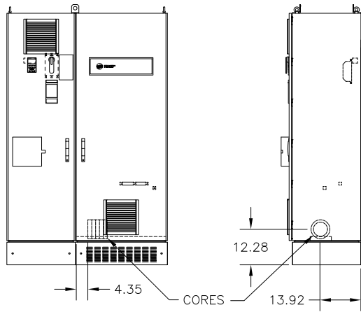
Figure 4. AFDG Remote-Mounted Drive (Frame E2)
