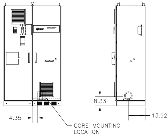
Figure 4. AFDG Remote-Mounted Drive (Frame E2)
