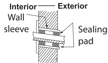
Figure 3. Protective pipe sleeve
