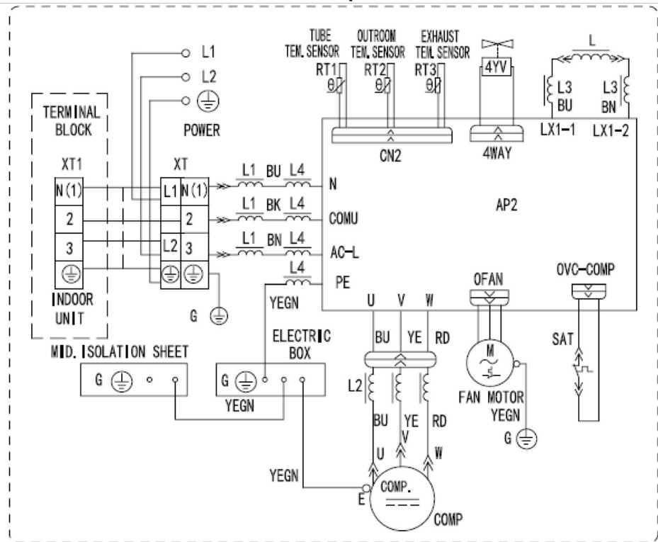
Figure 17. 4TYK4518A1 / 4TYK4524A1 Cooling Only Outdoor units
