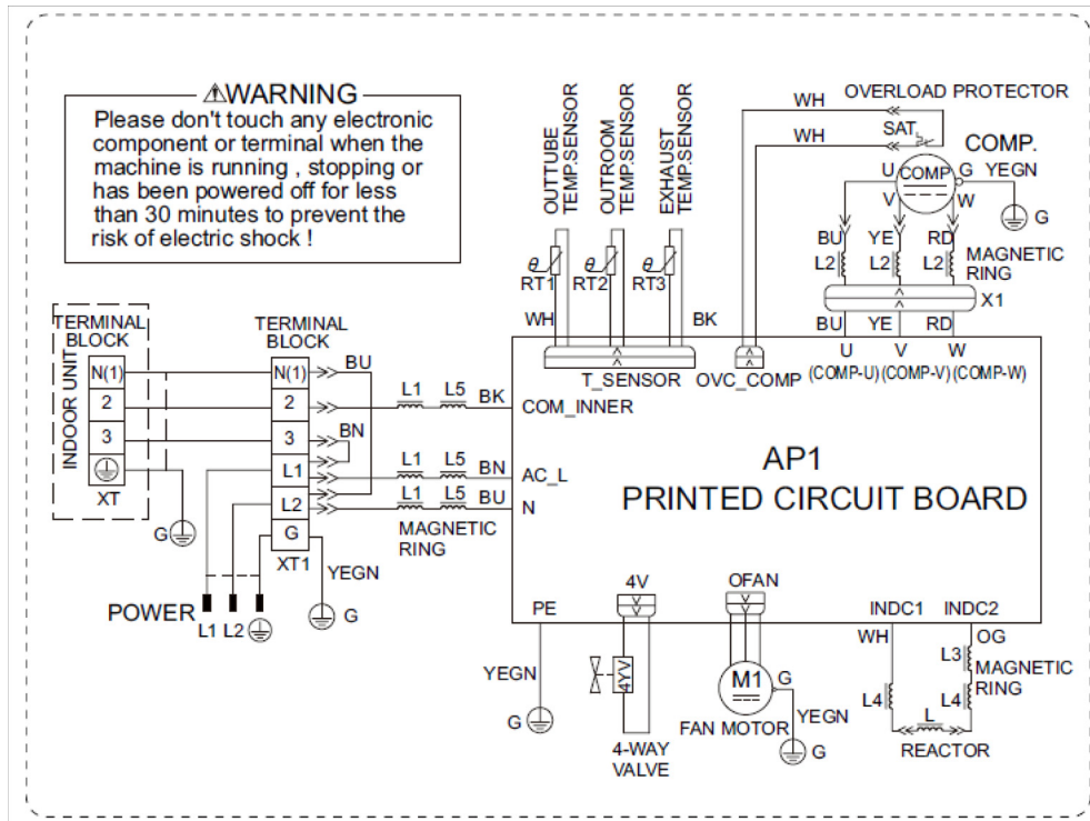
Figure 18. 4TXK4518A1 / 4TXK4524A1 Heat Pump Outdoor Units
