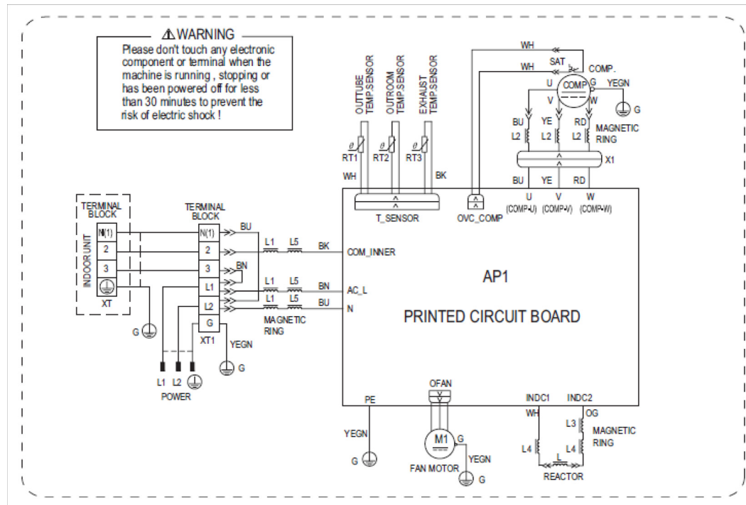
Figure 17. 4TYK4518A1 / 4TYK4524A1 Cooling Only Outdoor units
