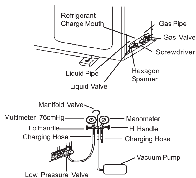
Figure 9. Vacuum Pump and Leak Inspection
