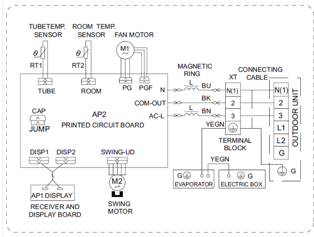
Figure 12. 4MYW4518A1 Cooling Only Indoor U./ 4MXW4518A1 Heat Pump Indoor U.
