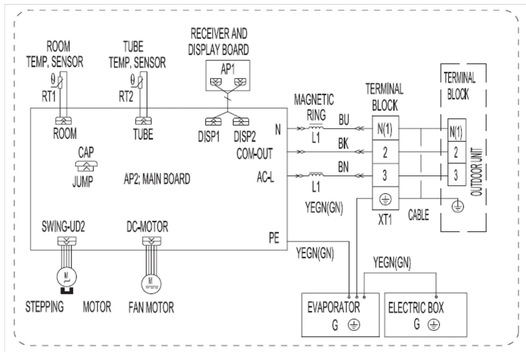
Figure 13. 4MYW4524A1 Cooling Only Indoor Units
