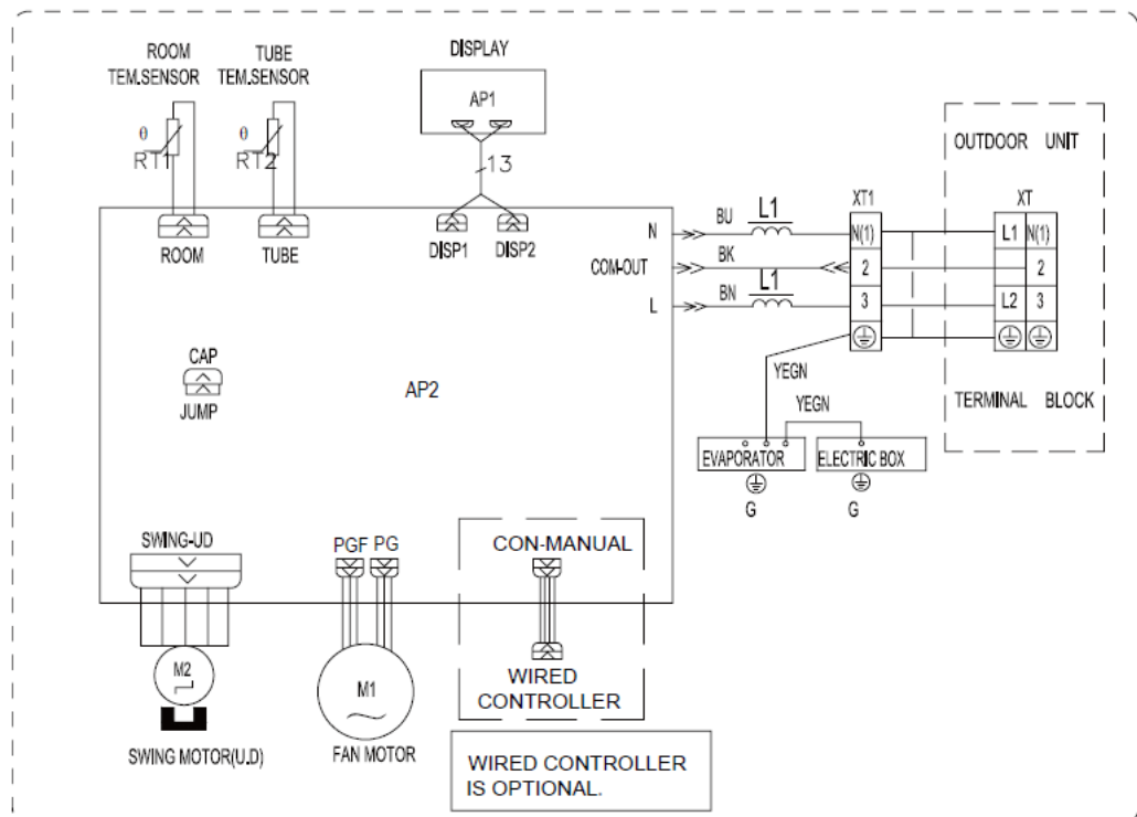
Figure 11. MYW4509A1 4MYW4512A1 Cooling Only Indoor U.-- 4MXW4509A1 4MXW4512A1 Heat Pump Indoor U.
