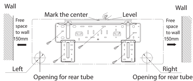
Figure 1. Mounting Plate Installation
