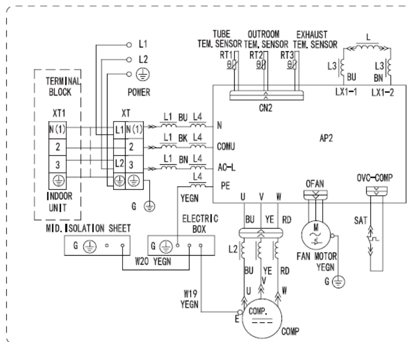
Figure 15. 4TYK4509A1 / 4TYK4512A1 Cooling Only Outdoor Units
