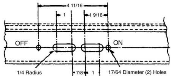
Figure 1-3 Flange Drilling Plan For Handle and Interlock Blade Mounting Dimensions
