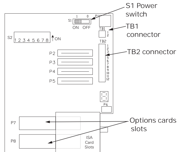
Figure 1. BCU main logic board (BMTW shown)
