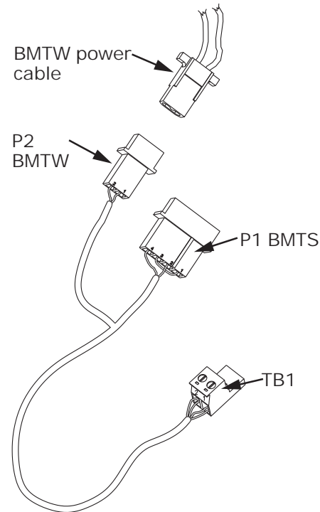
Figure 3. BMTW/BMTS power cable adapter
