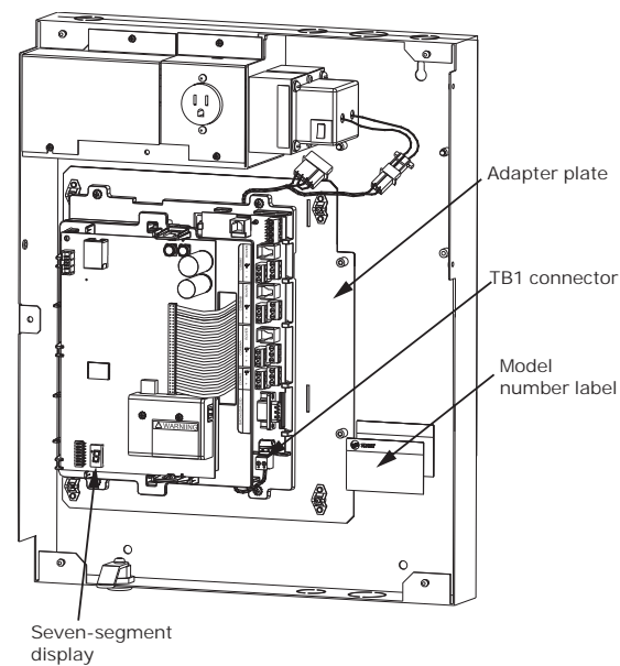
Figure 6. Completing the BMTX retrofit installation (power connection is for the BMTW, not the BMTS)
