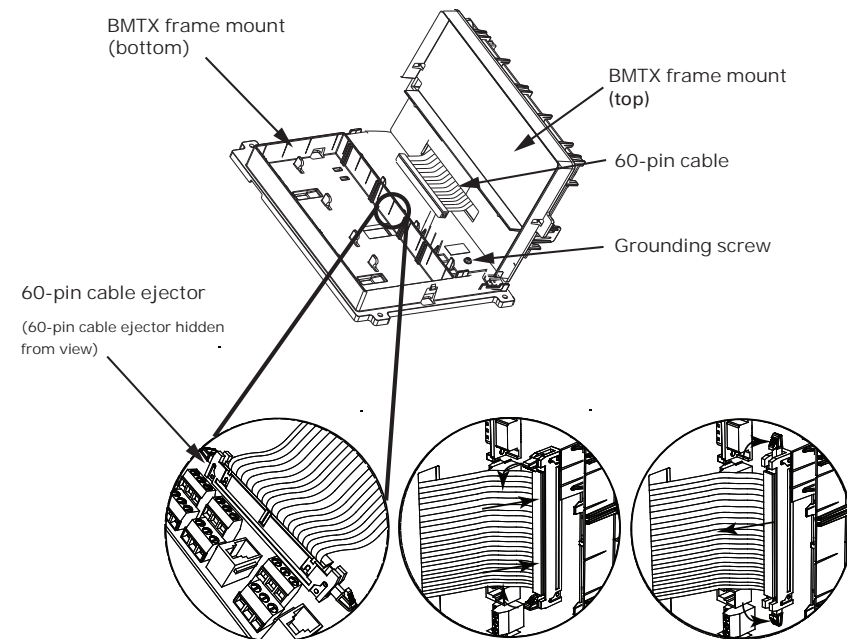
Figure 5. Accessing the grounding screw
