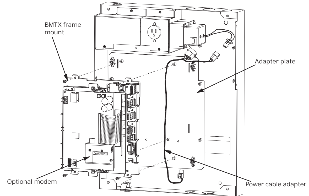
Figure 4. Installing the BMTX frame mount
