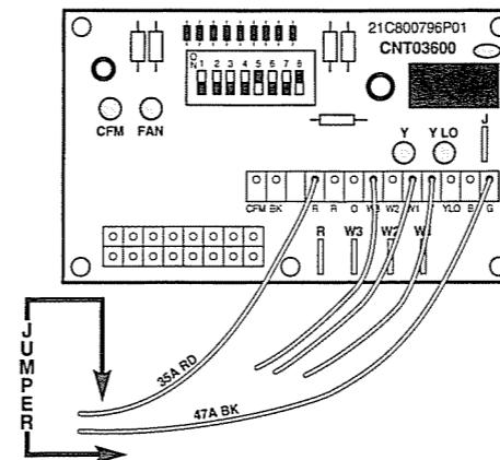
Package Unit Motor Control Board (ECMC)
