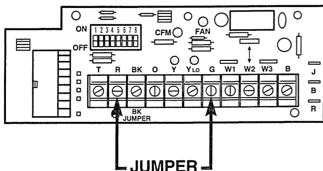
Package Unit Motor Control Board (ECMC)
