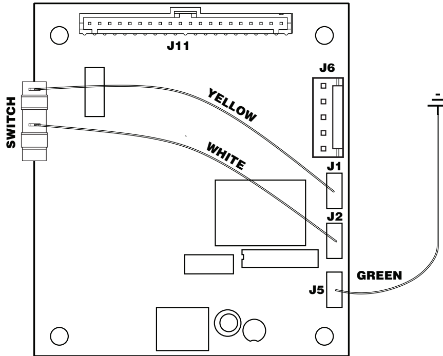
TYPICAL CONTROL BOARD
