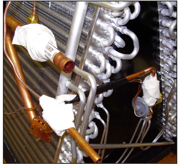
Figure 10 - Using wet rags
