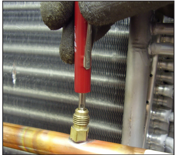
Figure 8 - Removing Schrader core
