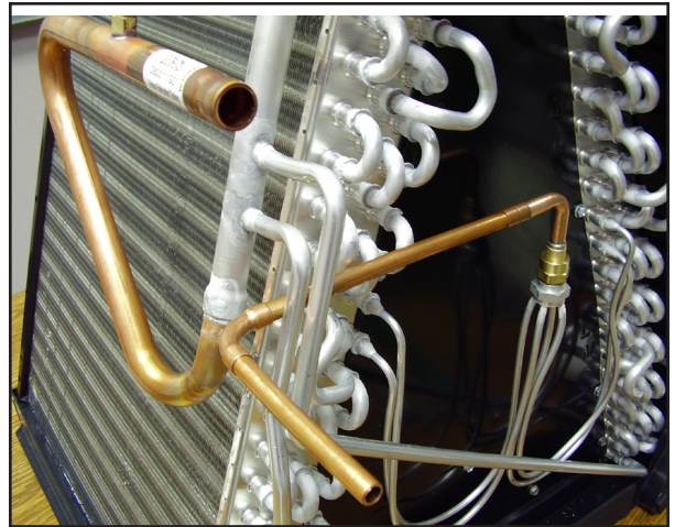
Figure 13 - Field fabricated liquid line
