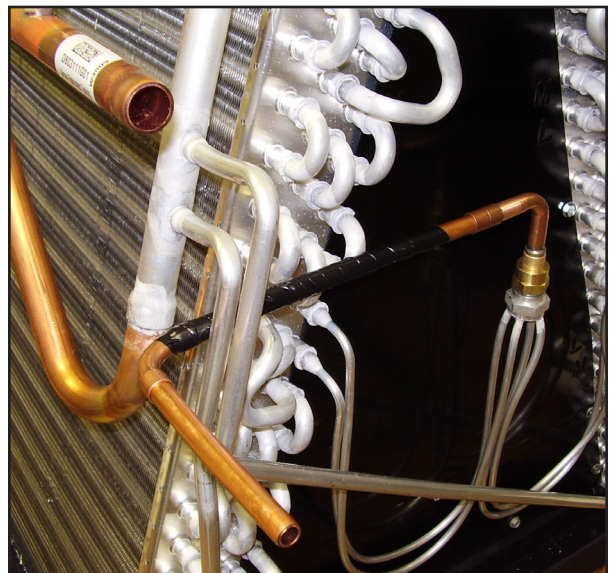
Figure 15 - Wrapping liquid line
