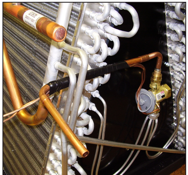
Figure 7 - Wrapping liquid line
