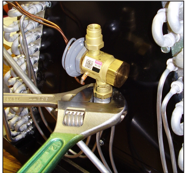
Figure 5 - Installing TEV
