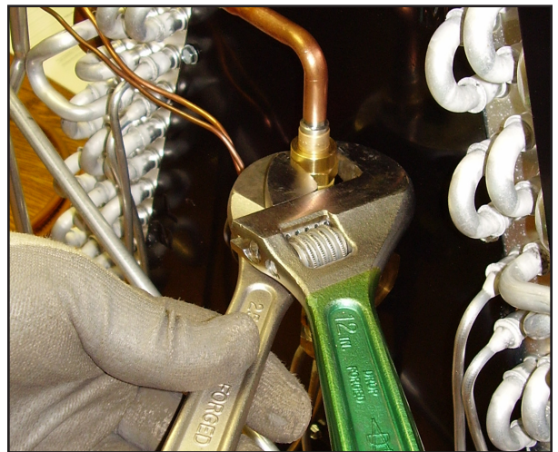
Figure 6 - Connecting liquid line
