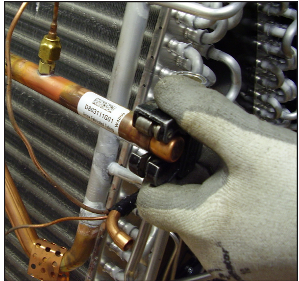
Figure 16 - Cutting off end of suction line
