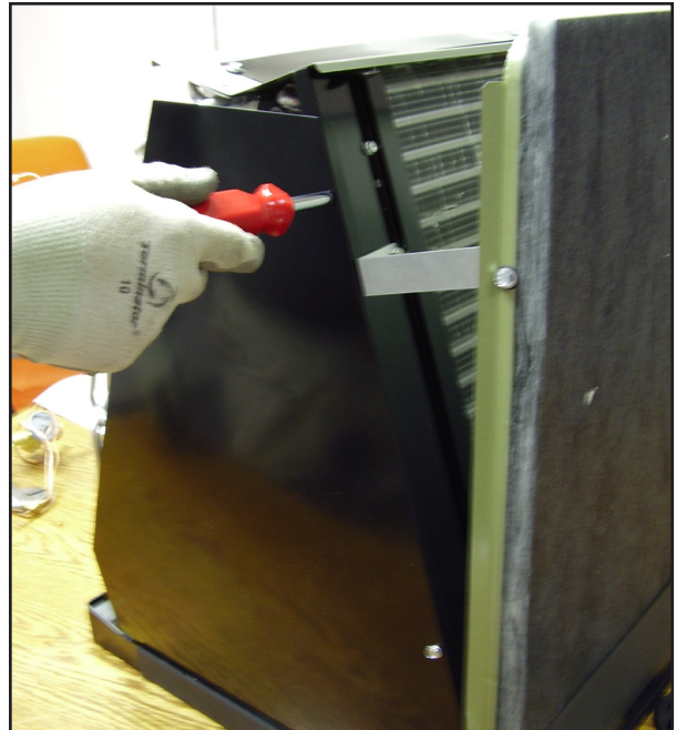
Figure 2 - Removing outer sheet metal cover
