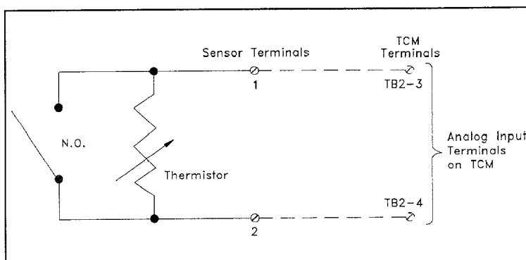
Figure 9 Schematic Diagram of Room Sensor with Override "ON" Switch
