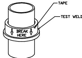
DETAIL 'E'
