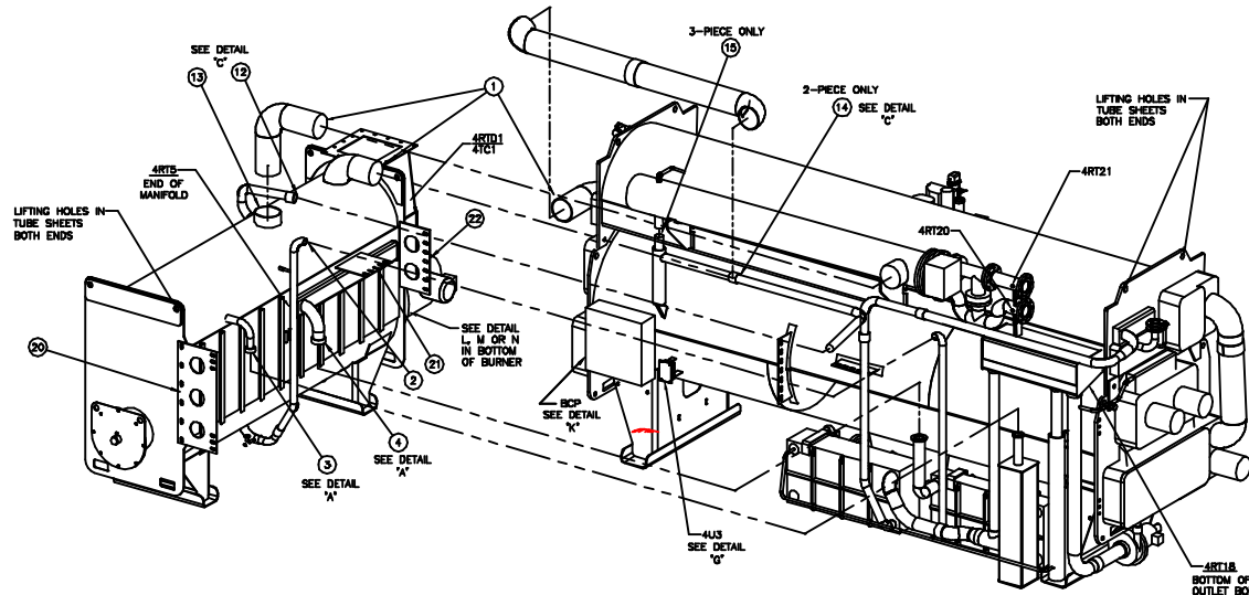
2-PIECE SPLIT (DIRECT FIRED GENERATOR & GEN/COND-EVAP/ABS)
