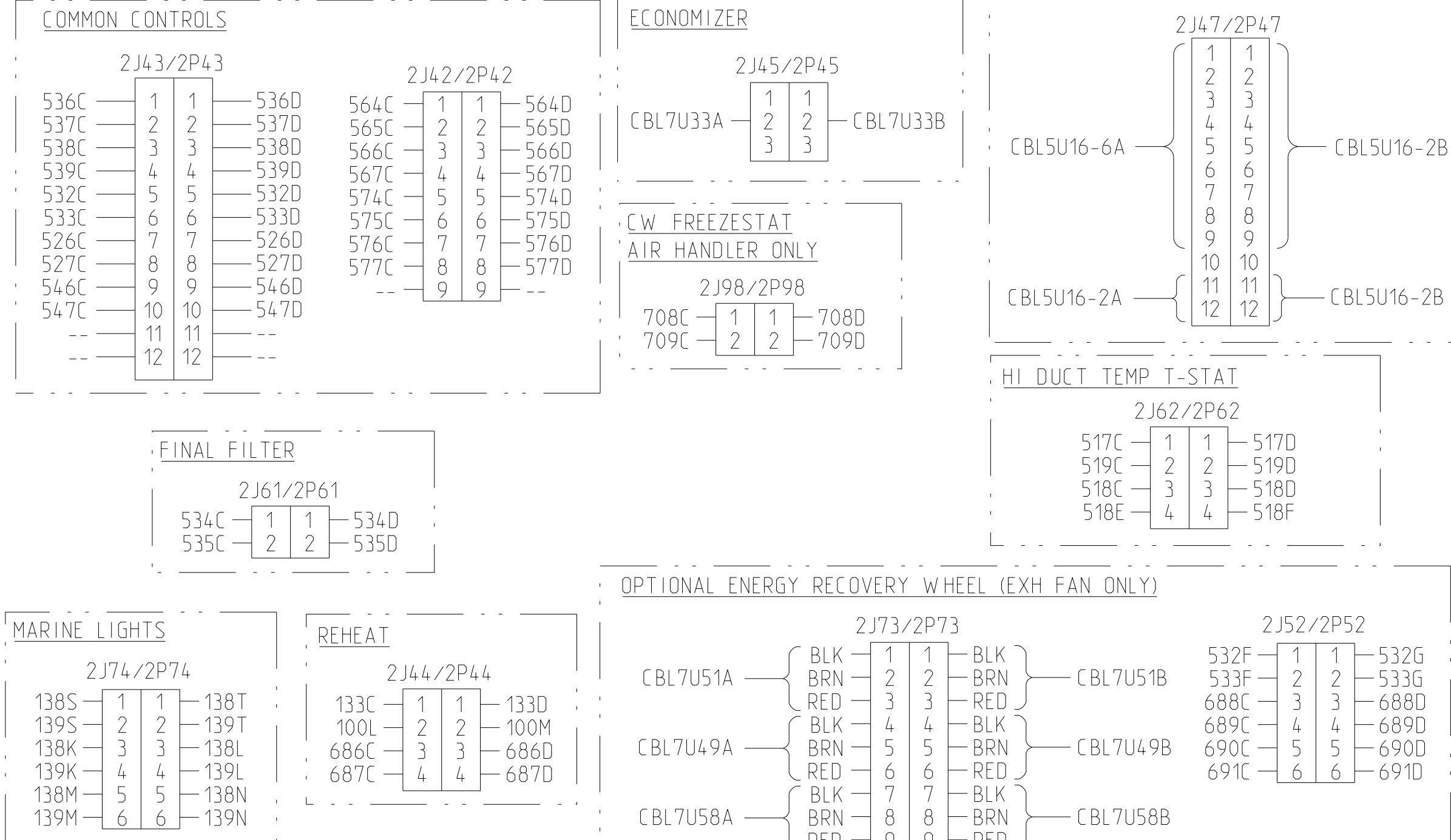
INSET 2H - 2PC JUNCTION BOX (CONTROLS)
