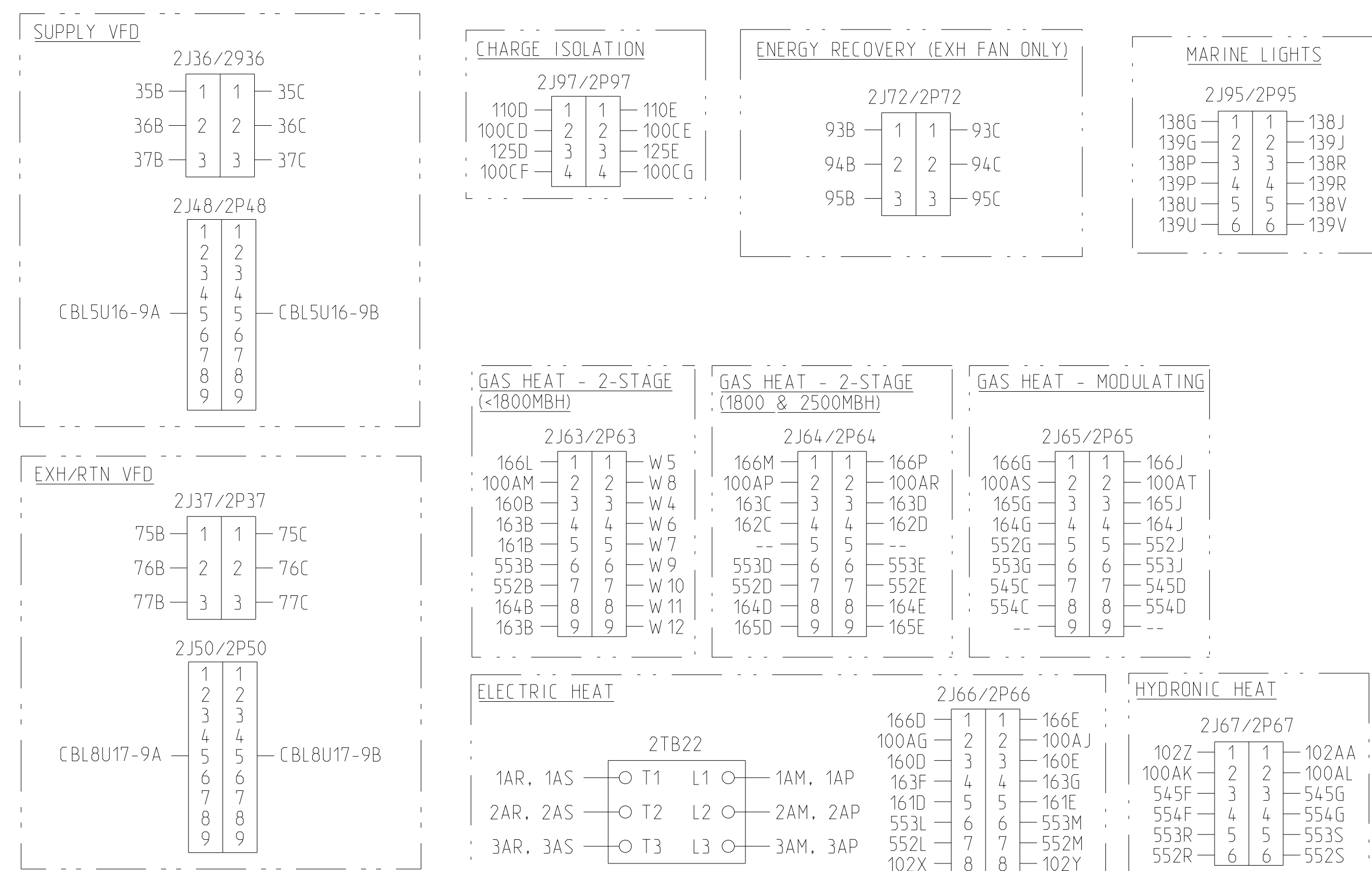
INSET 2G - 2PC JUNCTION BOX (POWER)
