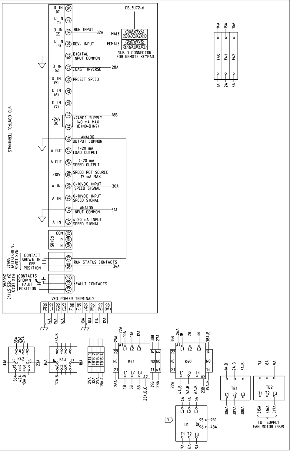
3U72 SUPPLY VFD ASSEMBLY
