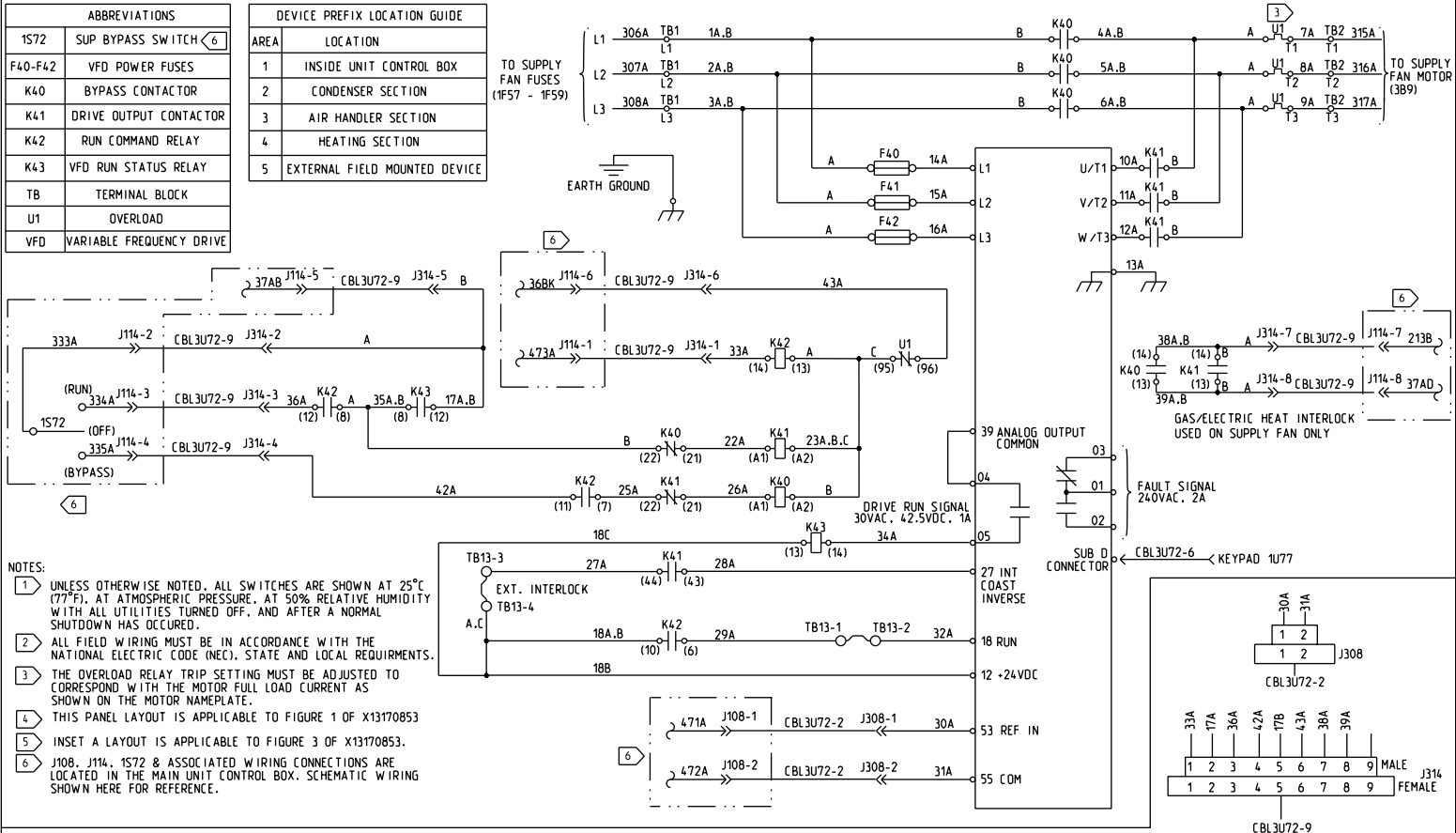
3U72 SUPPLY VFD ASSEMBLY
