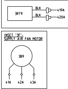
INSET "3M"- SUPPLY AIR TEMP SENSOR
