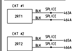
INSET "3C"- SAT COND TEMP SENSOR
