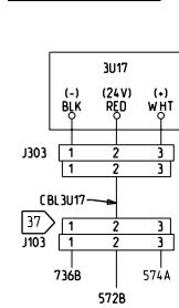
INSET "3S"- 1GV OPTION
