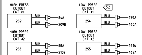
INSET "3D"- HIGH AND LOW PRESSURE CUTOUTS
