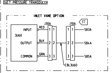
INSET "3T"- SUPPLY AIR DUCT PRESSURE TRANSDUCER
