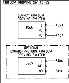
INSET "3R"- SUPPLY &amp; EXHAUST/RETURN AIRFLOW PROVING SWITCHES
