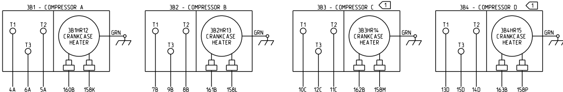
CIRCUIT NO. 2
