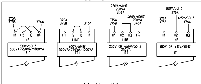
DETAIL "1B"
