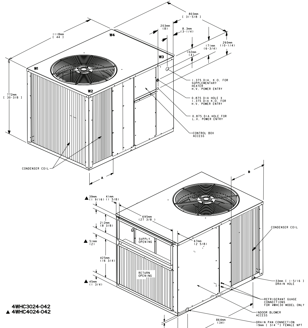
Figure 2. Dimensional Drawing
