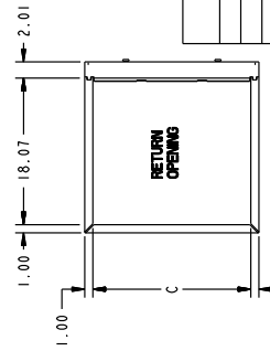
BOTTOM VIEW
