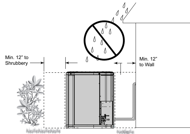
Figure 8. Do not install need water runoff
