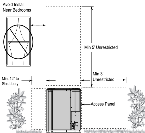
Figure 7. Ideal location shown
