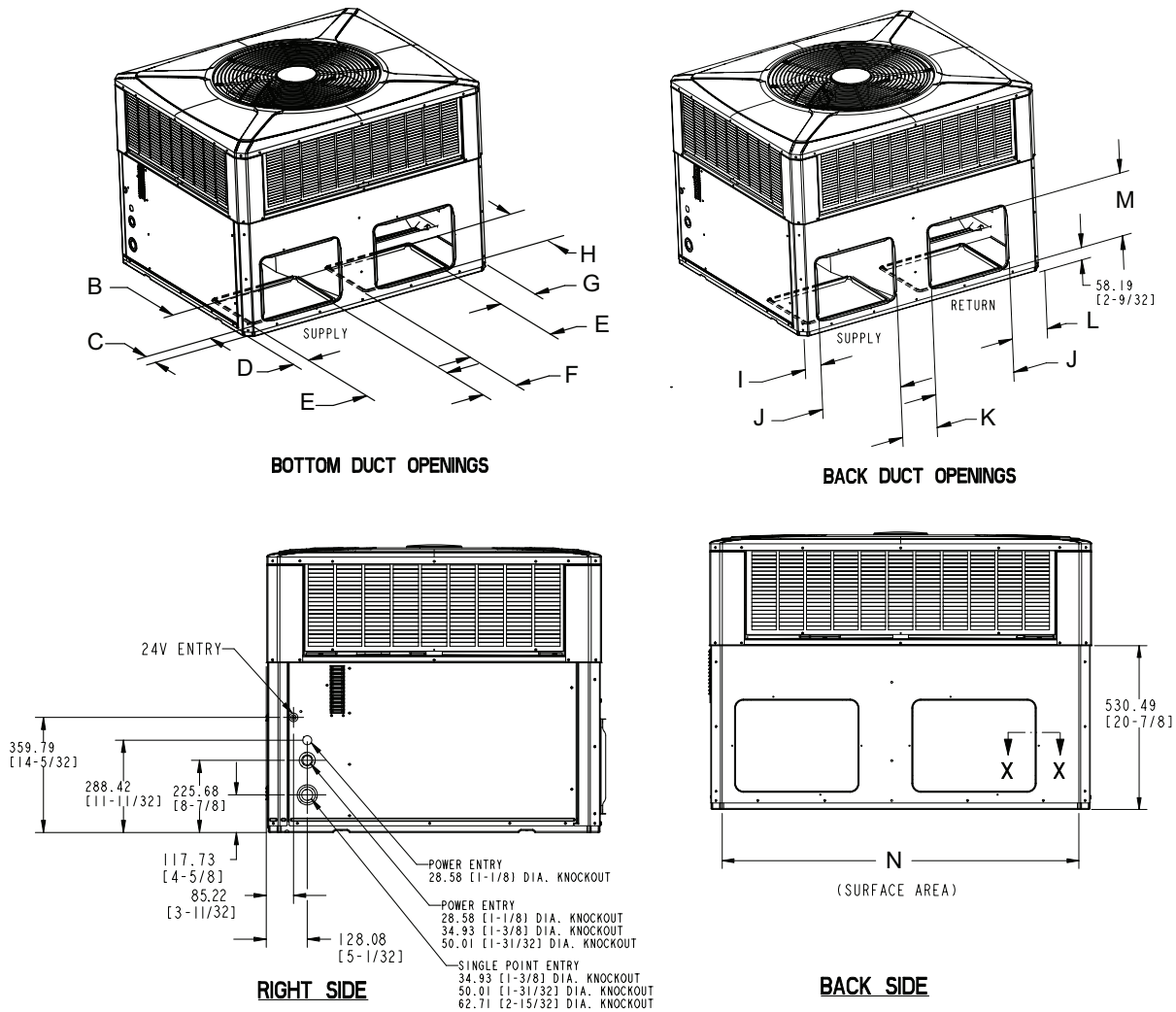
Figure 14. Bottom and back duct openings
