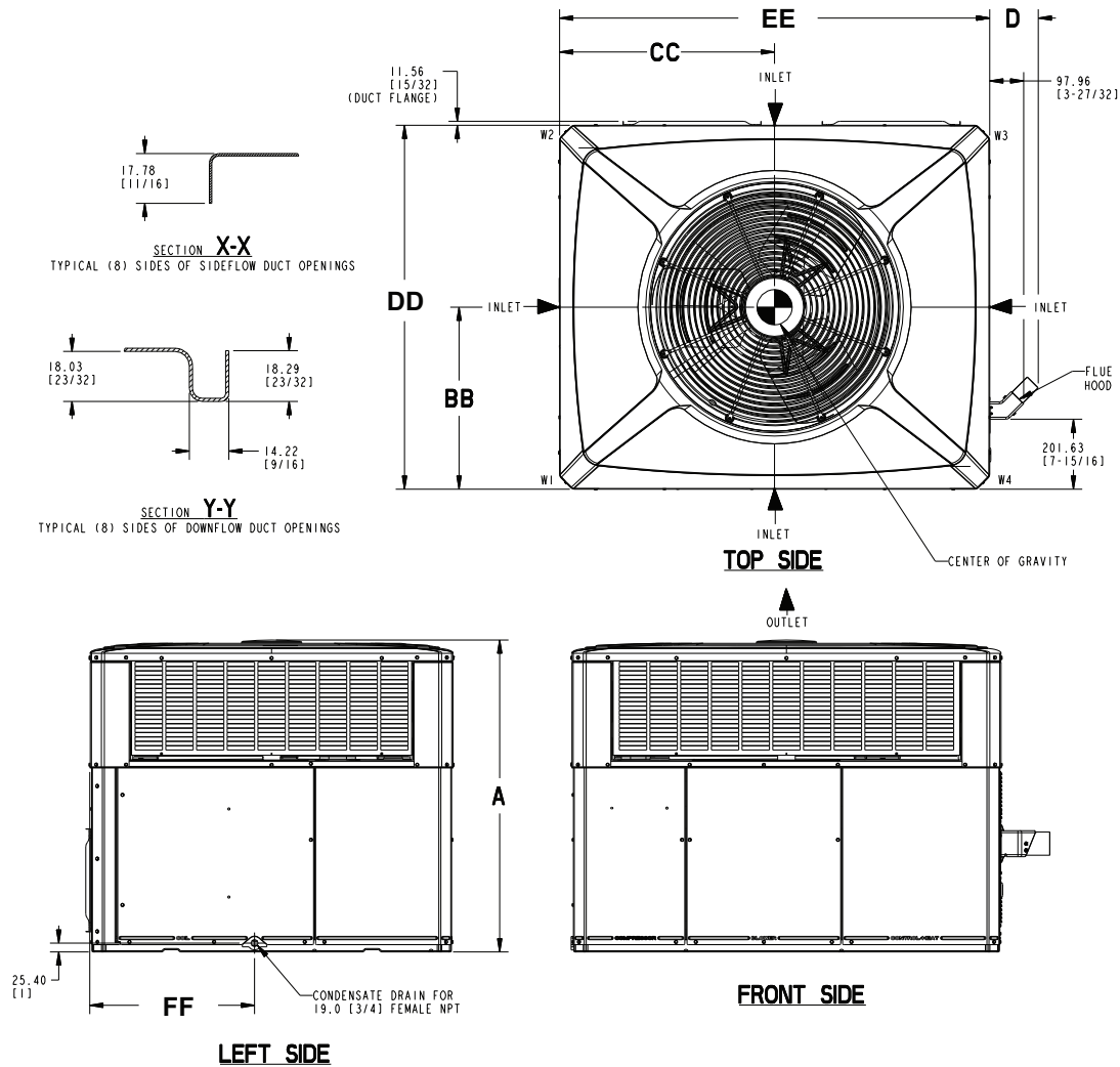
Figure 9. Space on sides requirements
