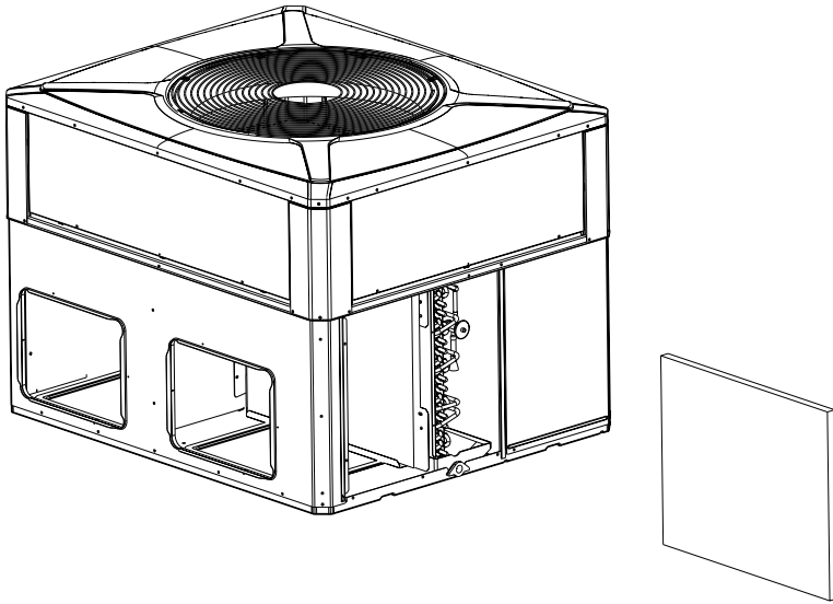
Figure 8. BAYACCDOR1A hinged filter access door (2.0 to 3.0 ton models) BAYACCDOR2A (3.5 to 5.0 ton models) (Replaces filter/coil access panel)
