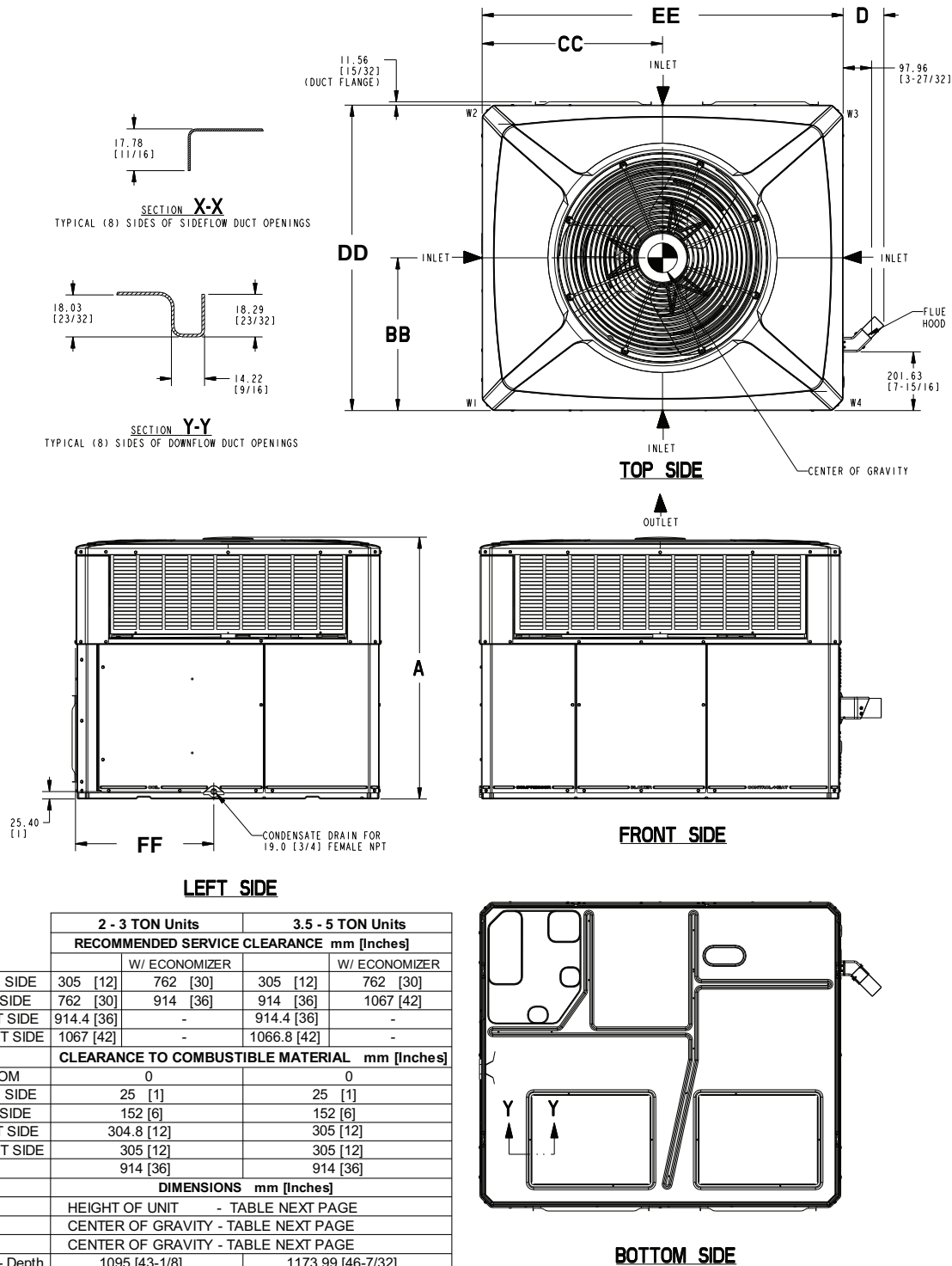
Figure 17. Space on sides requirements
