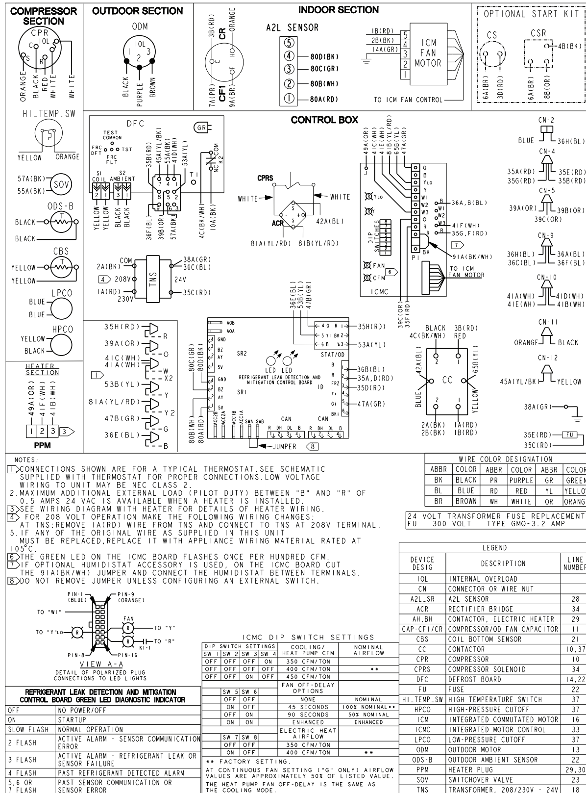
Figure 1. Models - 5WCZ5024A1, 5WCZ5030A1, 5WCZ5036A1, 5WCZ5042A1, and 5WCZ5048A1
