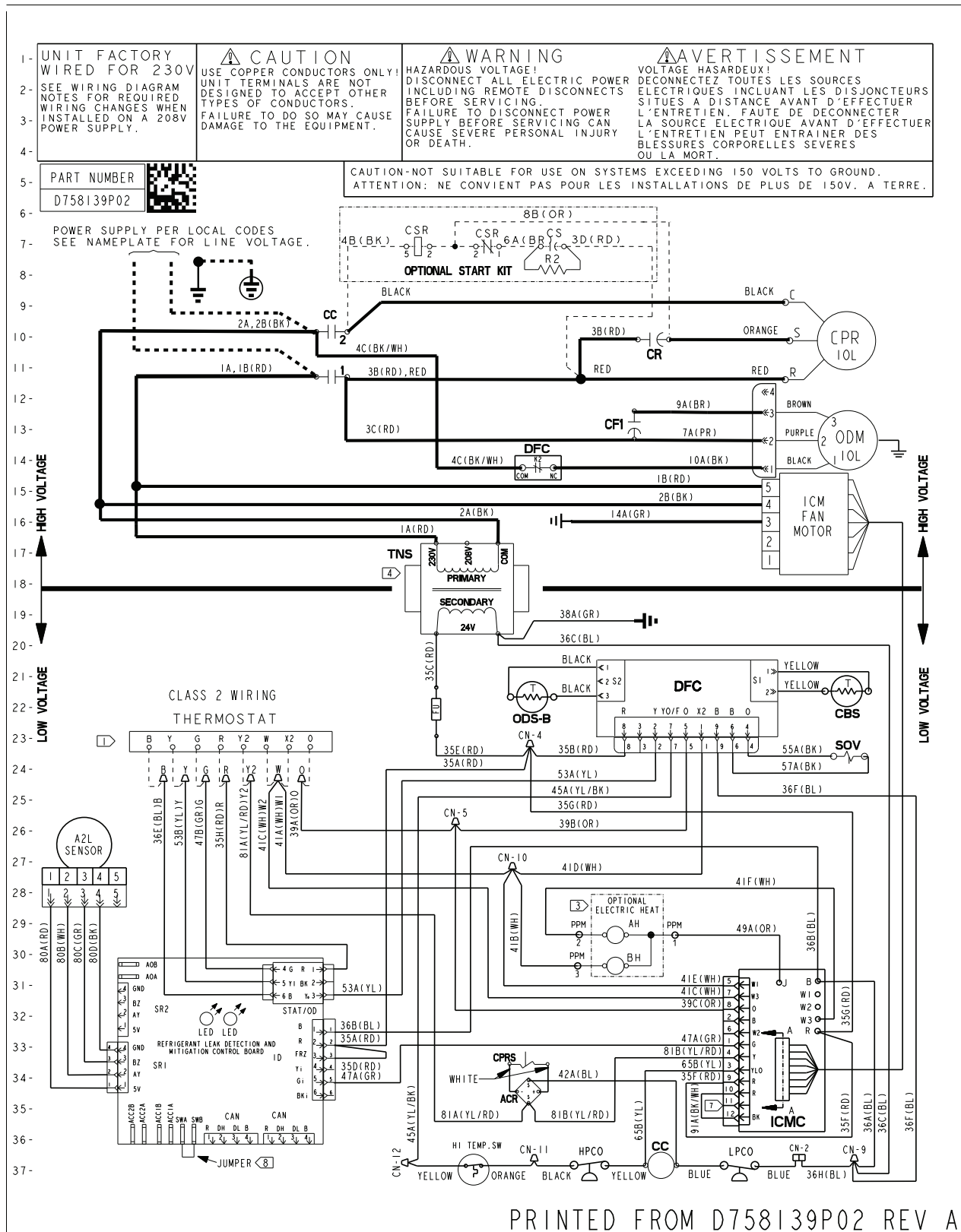
Figure 4. Model - 5WCZ5060A1
