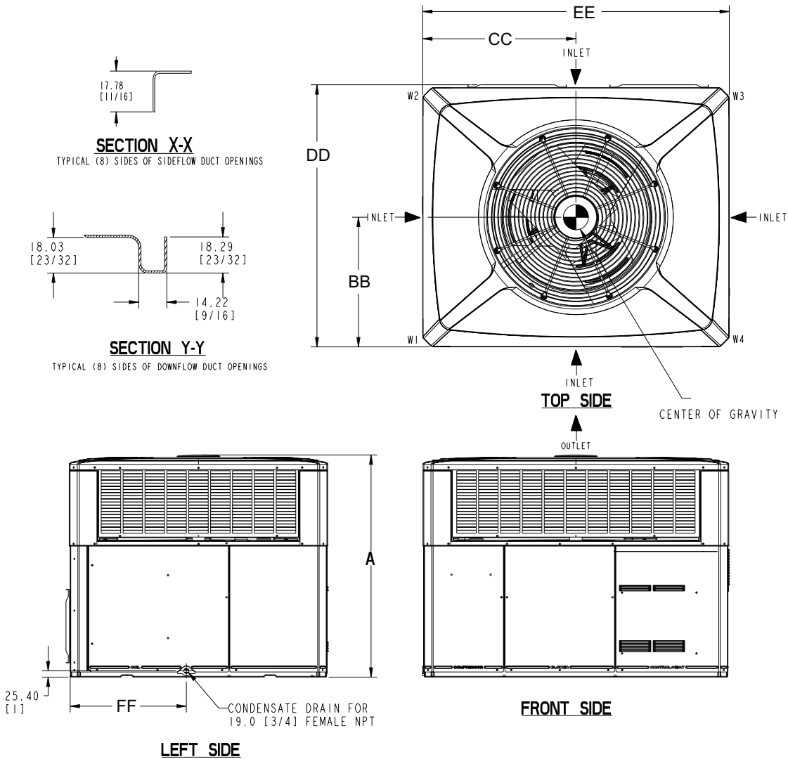
Figure 13. Space on sides requirements
