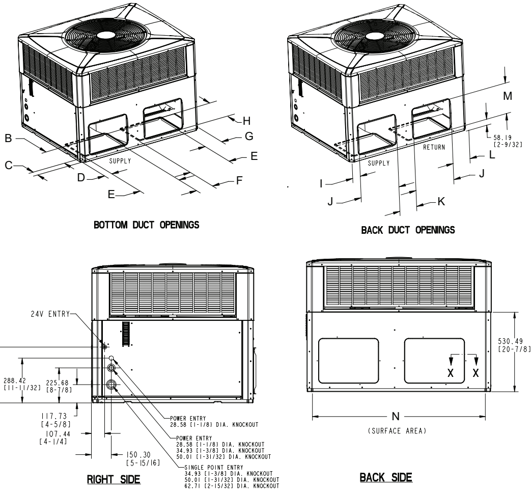
Figure 14. Bottom and back duct openings
