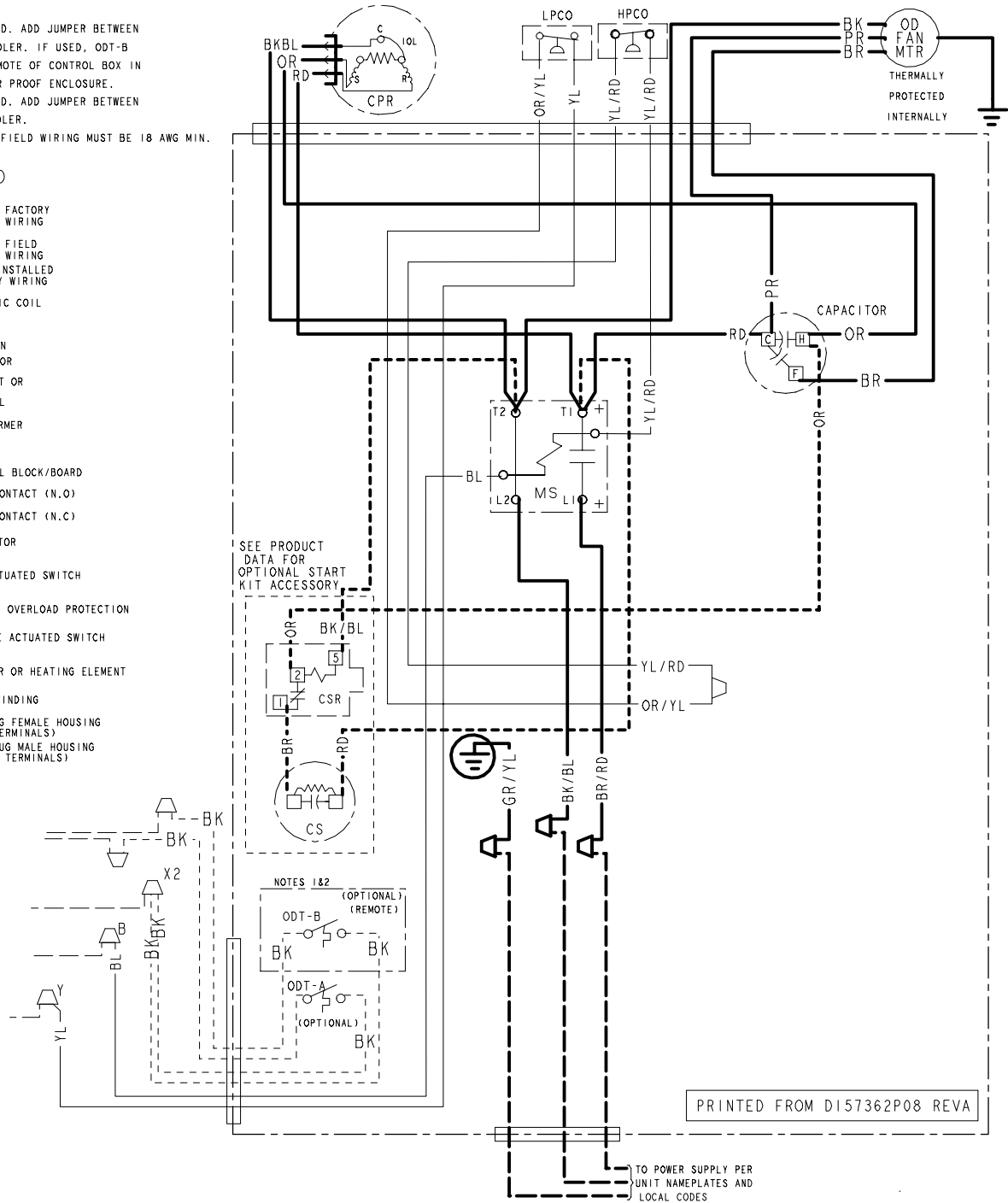
Figure 2. Models – A5AC5018, 024, 030, 036, 042, and 048
