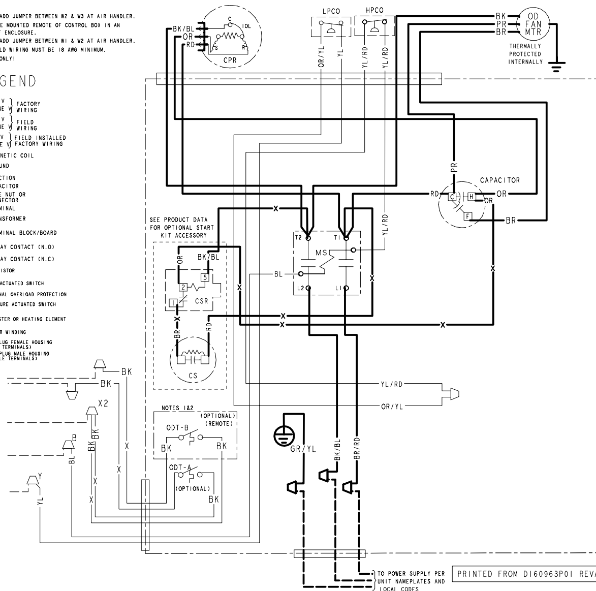
Figure 4. Model – A5AC5060
