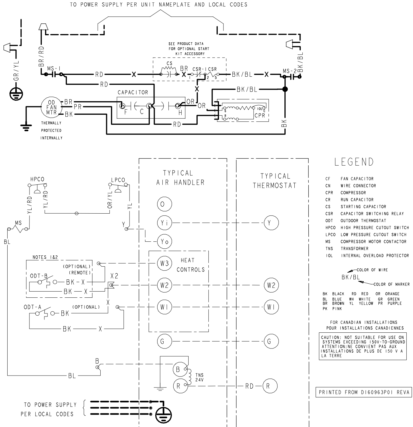
Figure 3. Model – A5AC5060
