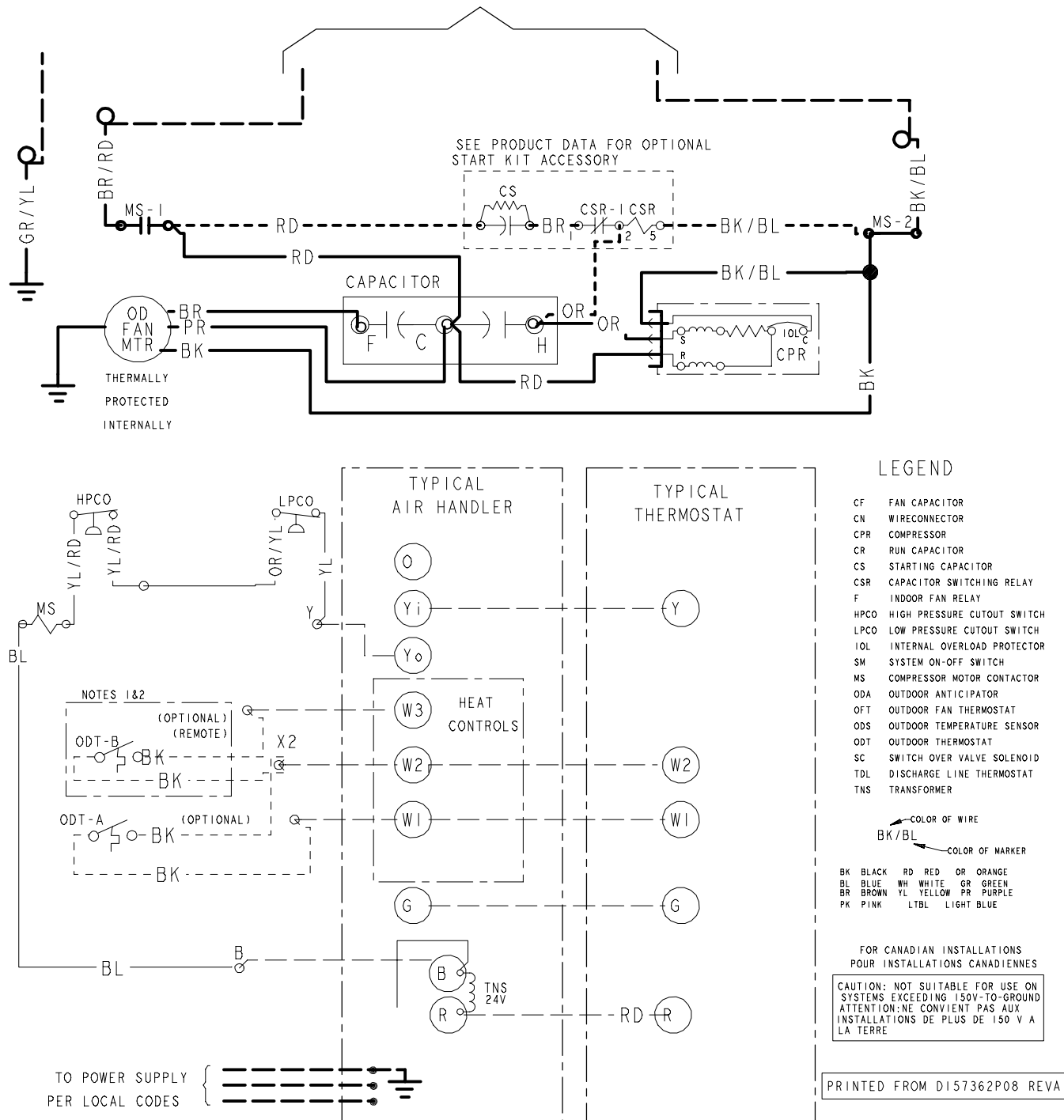
Figure 1. Models – A5AC5018, 024, 030, 036, 042, and 048
