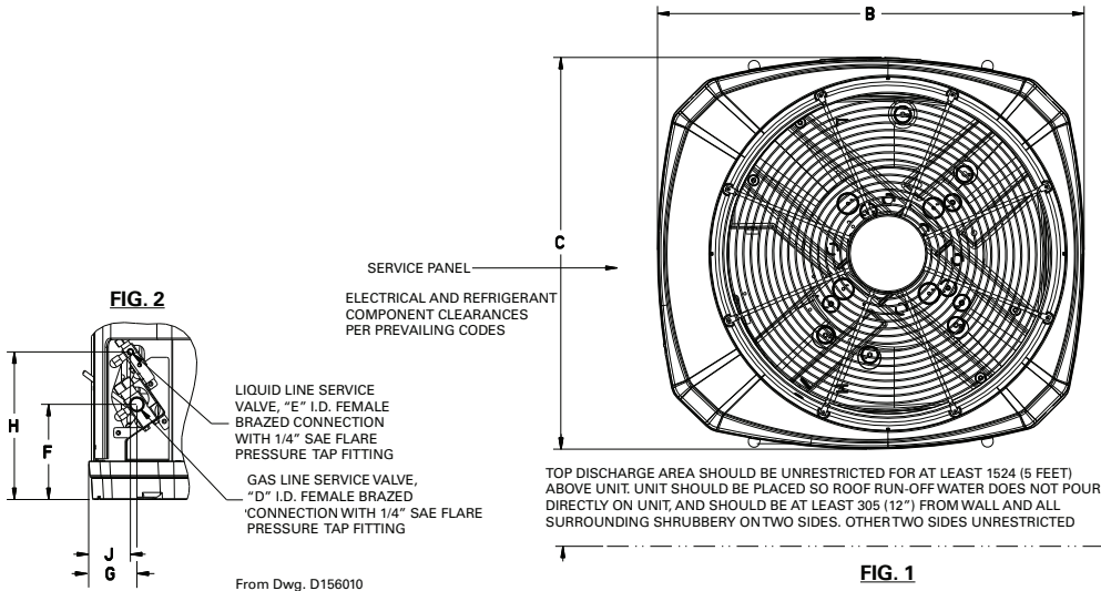
Figure 2. Dimensional drawing
