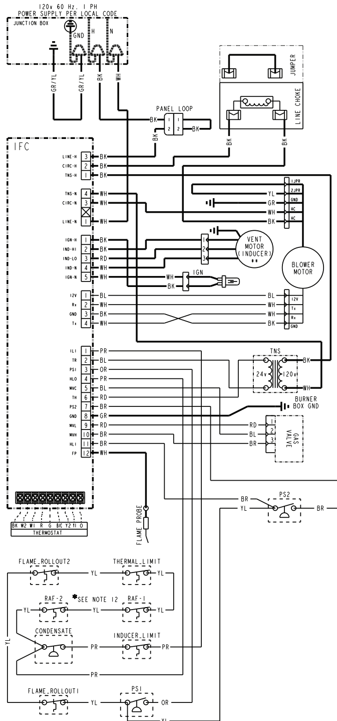
Figure 2. A952V - ladder diagram
