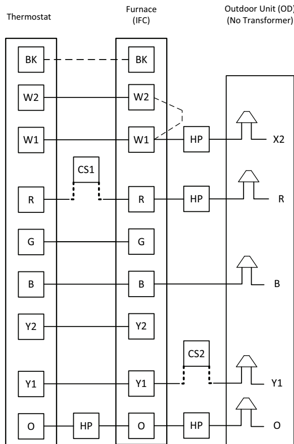
Figure 4. Field wiring diagram for A952V with single stage AC or heat pump with 2 stage airflow
