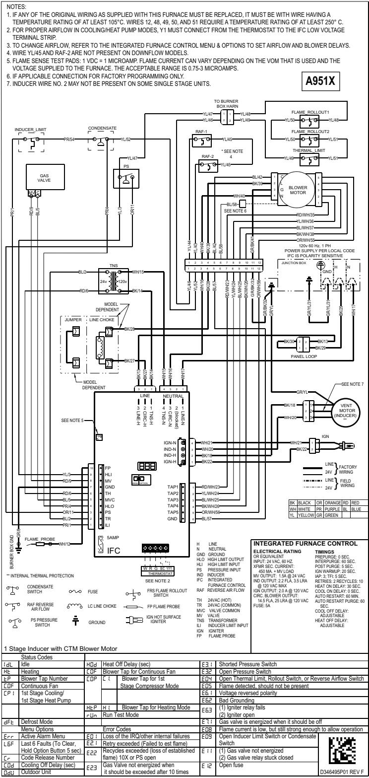
Figure 1. A951X wiring diagram
