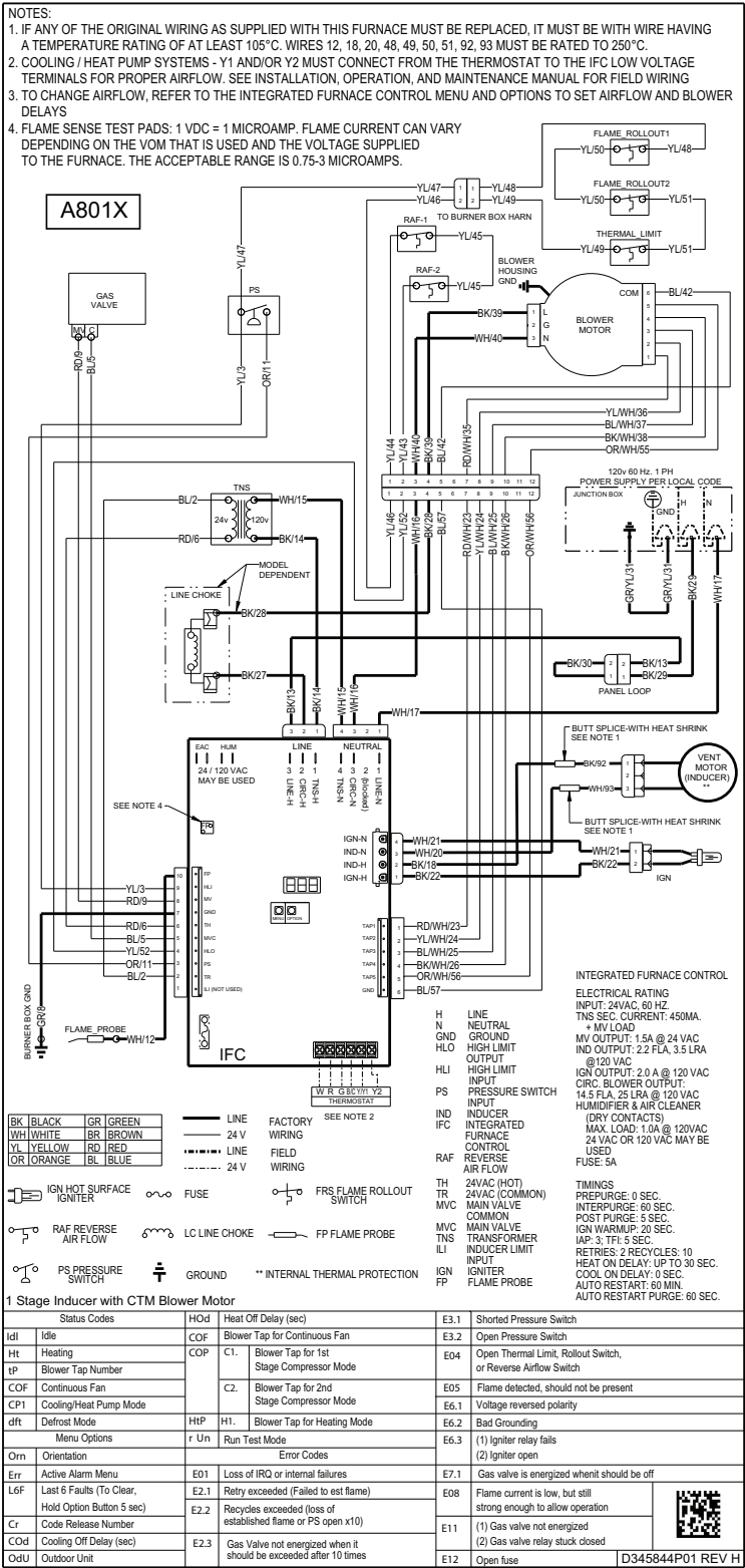
Figure 1. A801X — wiring diagram
