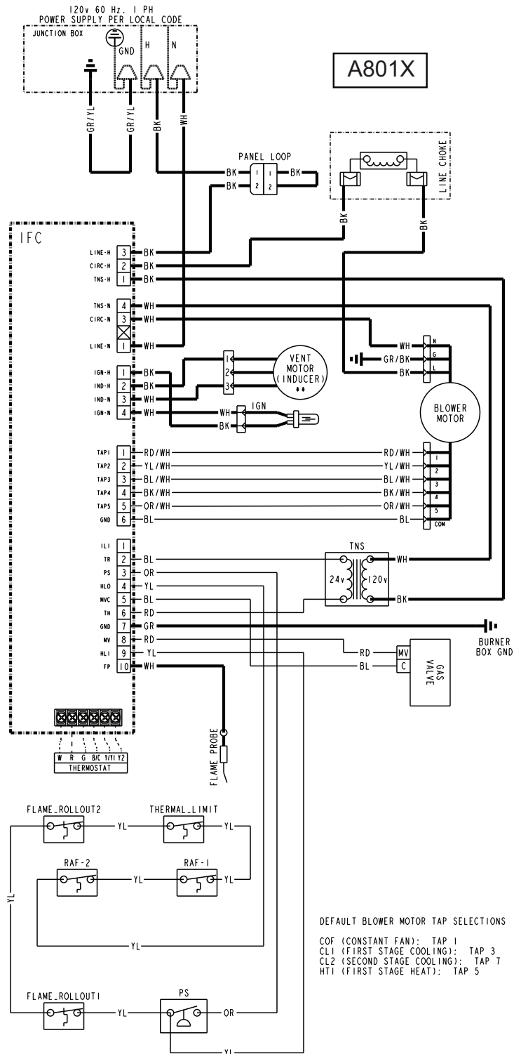
Figure 2. A801X — ladder diagram
