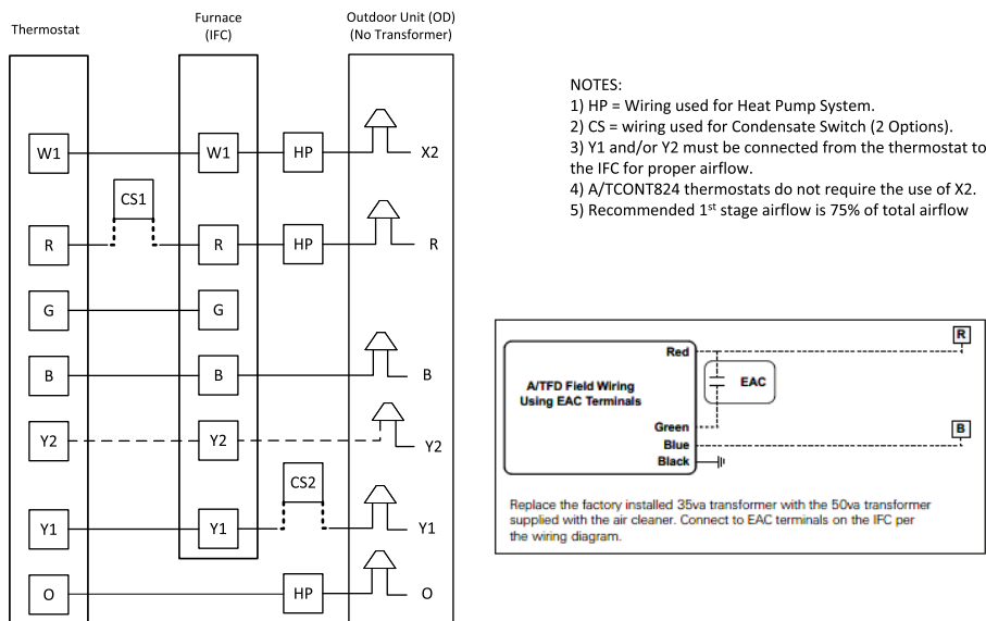
Figure 4. Field wiring diagram for A801X with single stage AC or heat pump with two stage airflow
