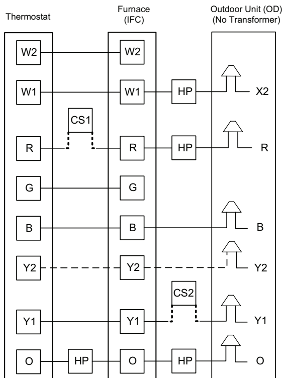
Figure 3. S9X2 with one or two stage AC or HP
