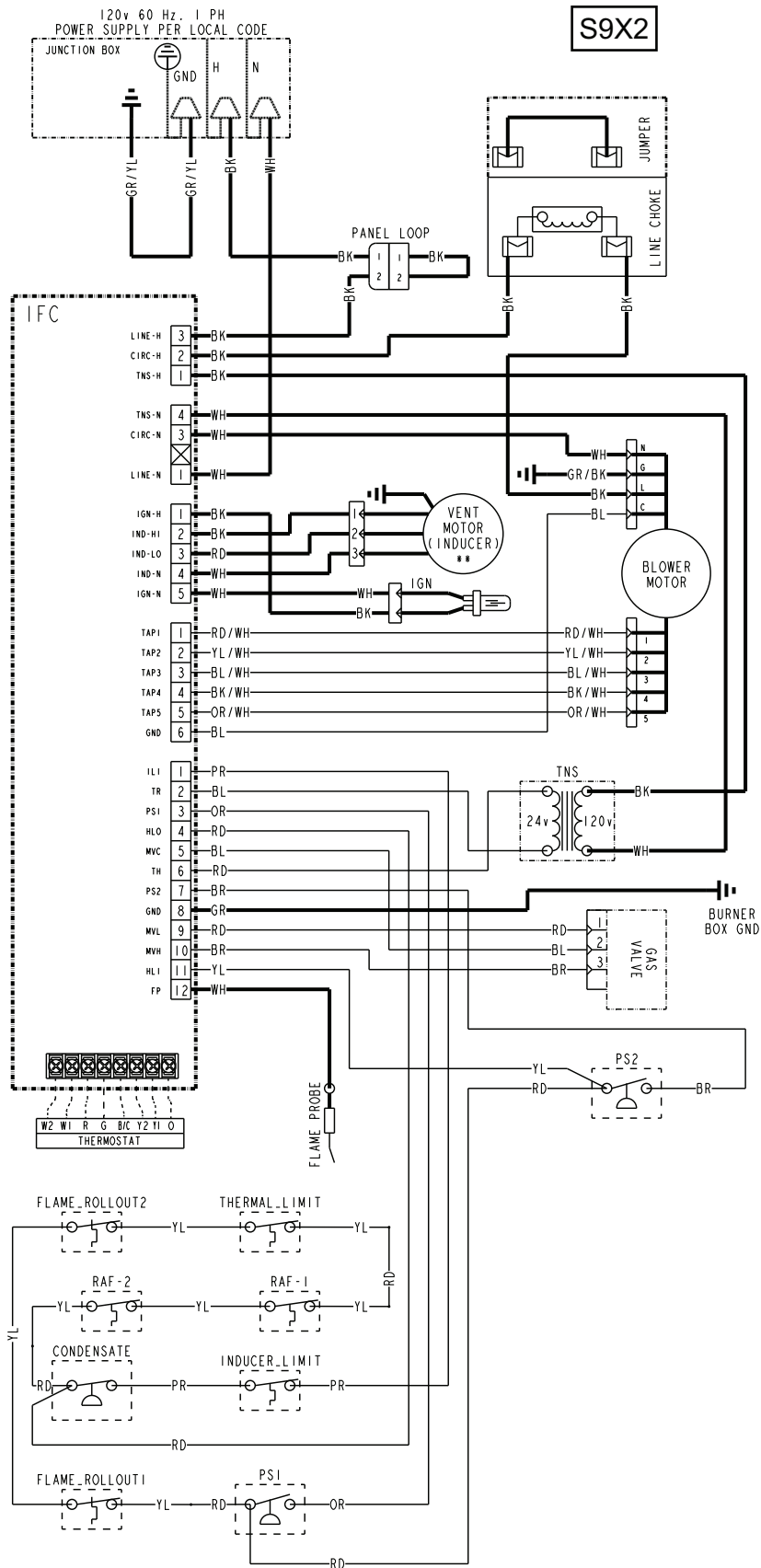
Figure 2. S9X2 ladder diagram
