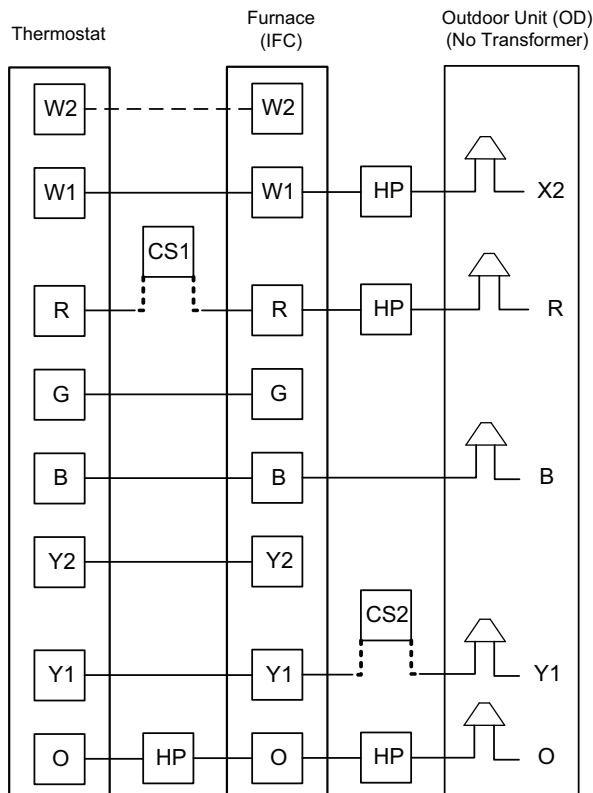
Figure 4. S9X2 with single stage AC or HP with two stage airflow
