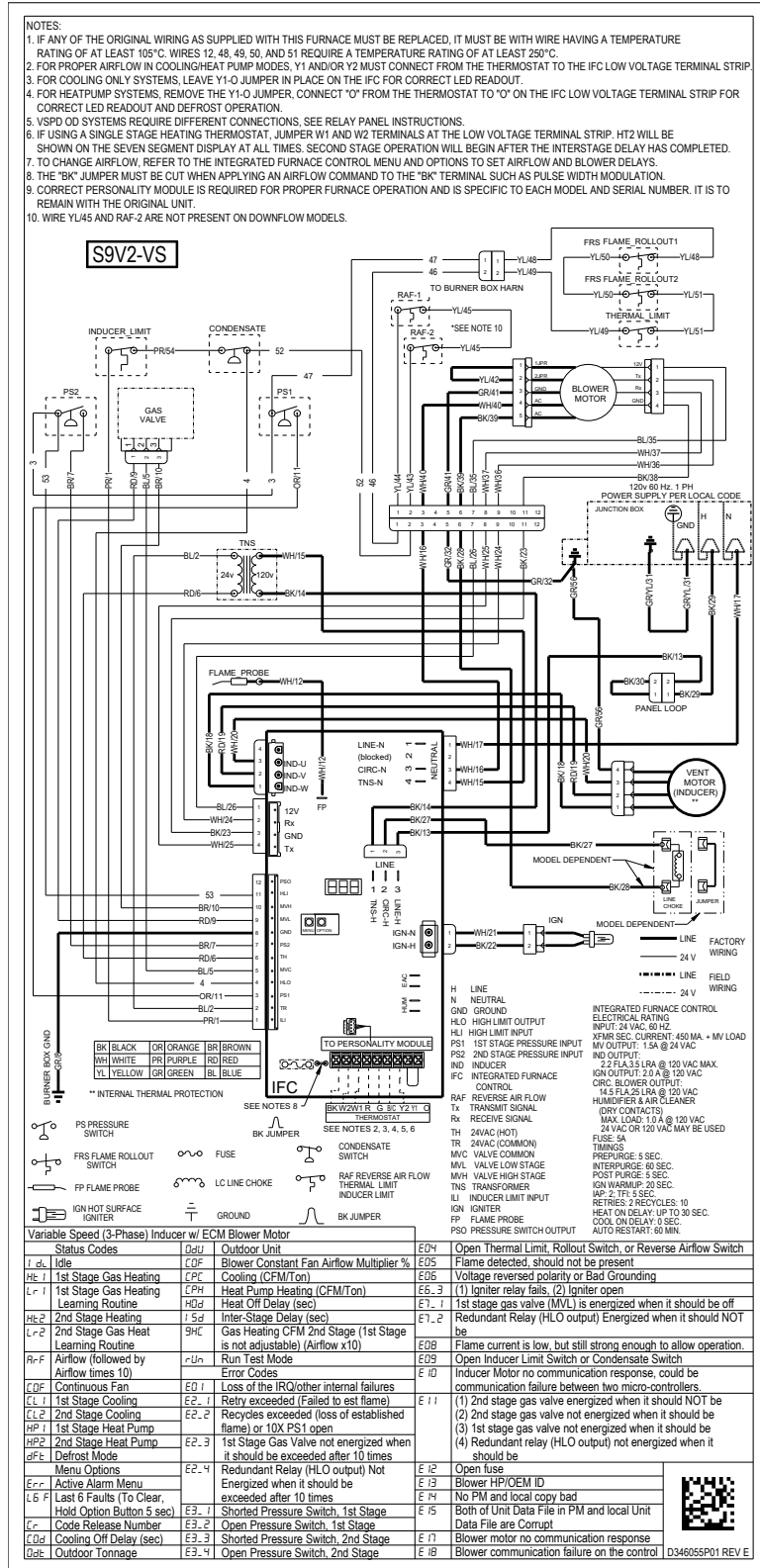
Figure 1. S9V2-VS wiring diagram
