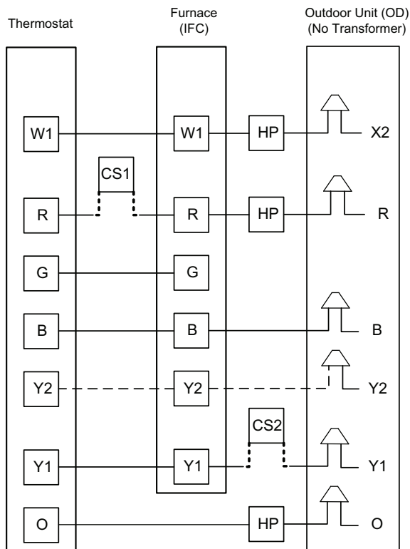
Figure 5. S9B1/S9X1 with one or two stage AC or HP
