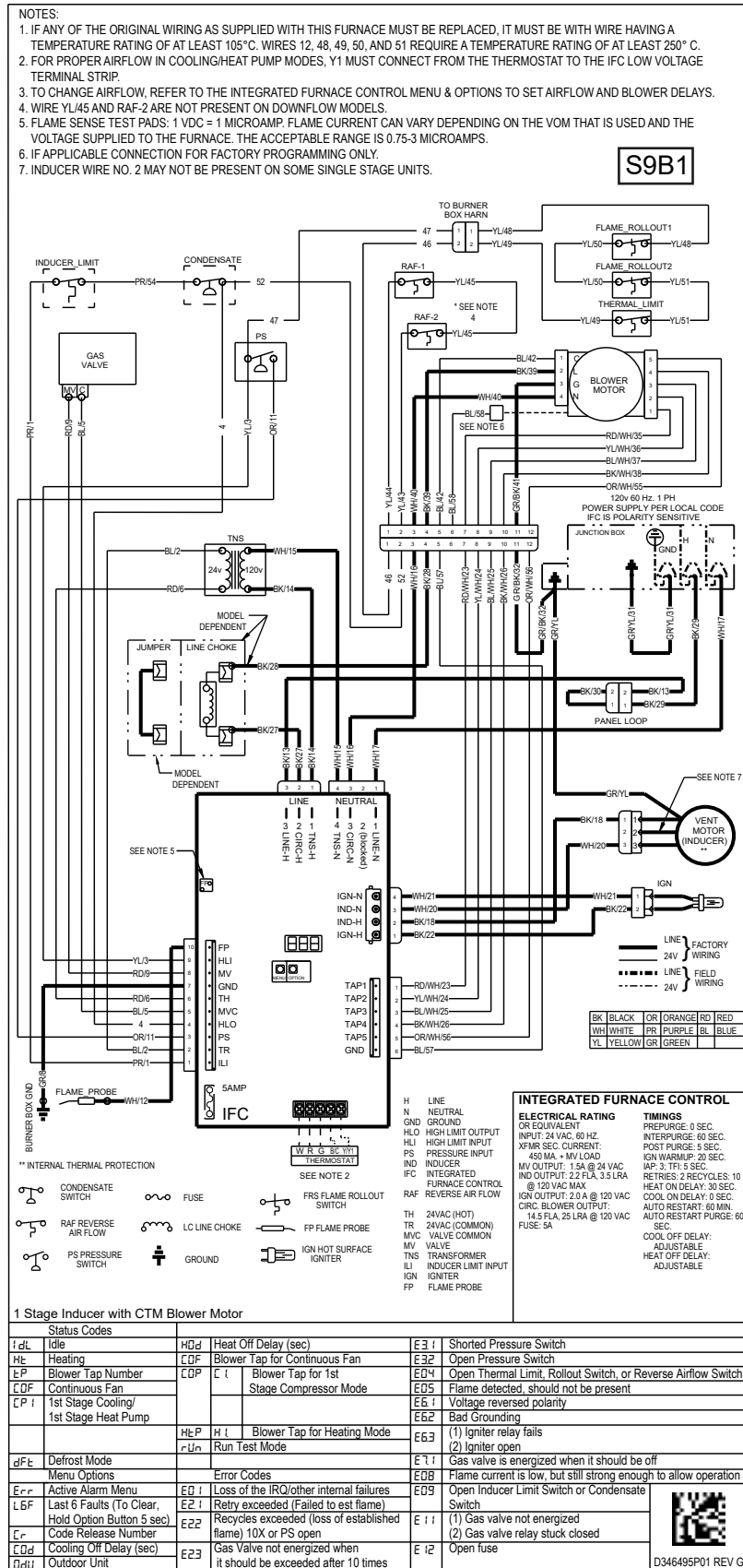
Figure 3. S9B1 wiring diagram
