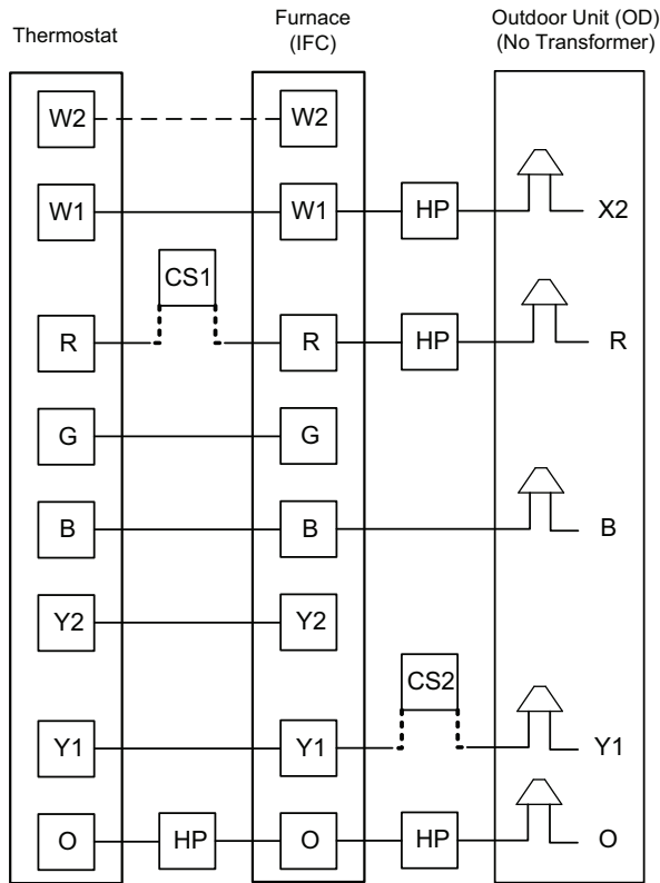
Figure 6. S9X1 with single stage AC or HP with two stage airflow
