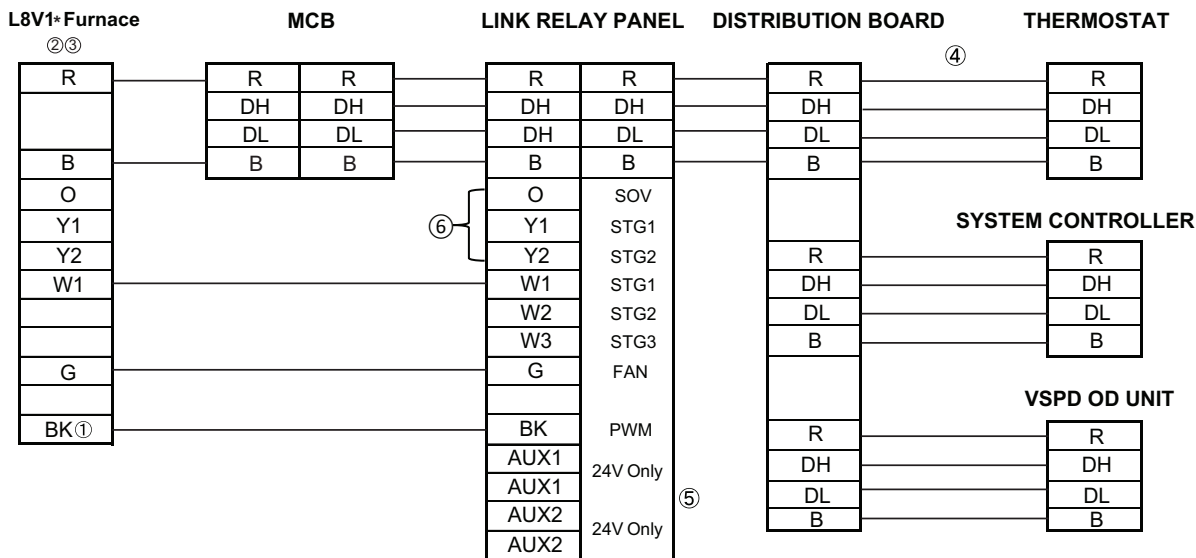
Figure 5. R454-B – link communicating vs heat pump or AC with non communicating L8V1 furnace
