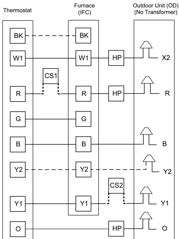
Figure 3. Field wiring for L8V1 with one or two stage AC or heat pump
