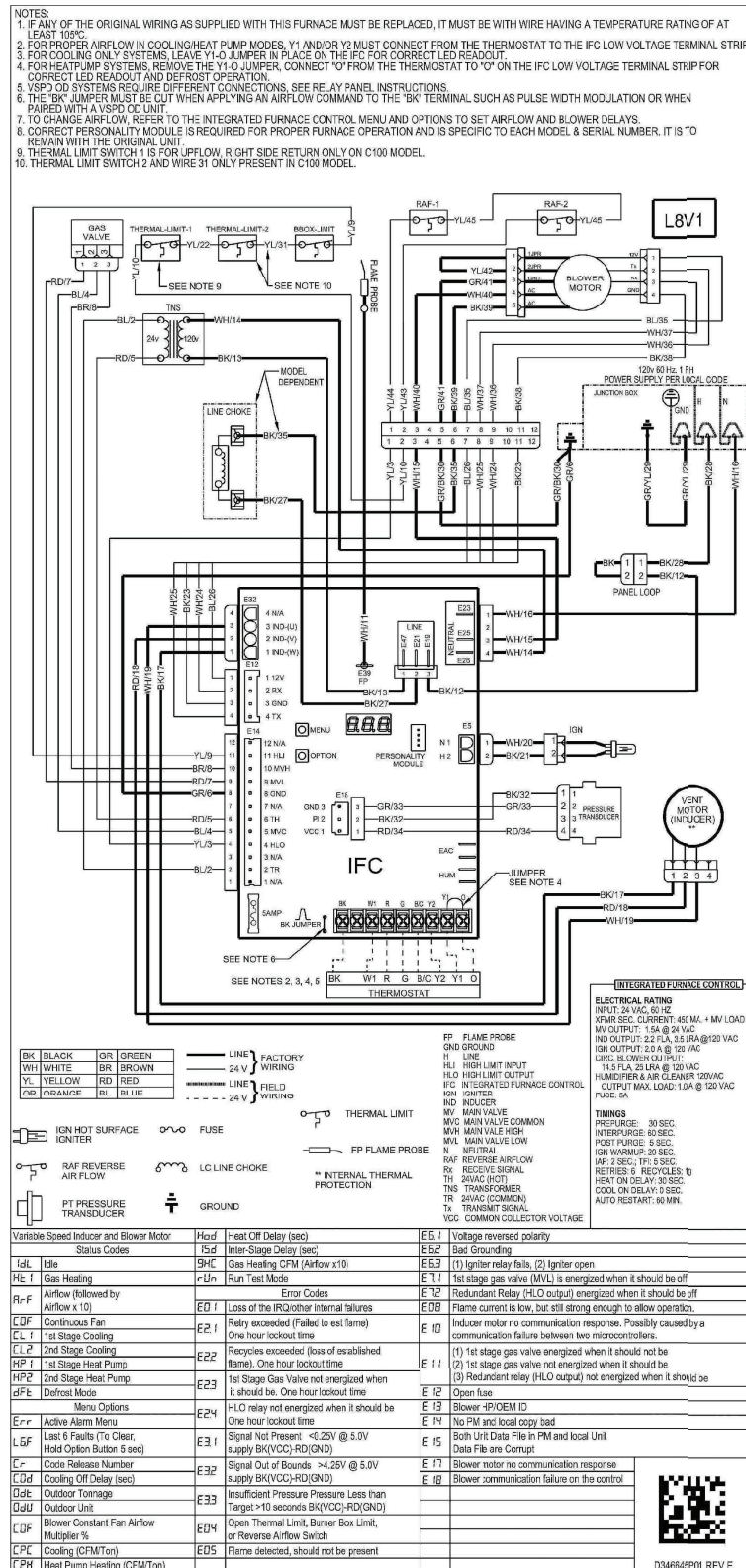
Figure 1. L8V1 – wiring diagram
