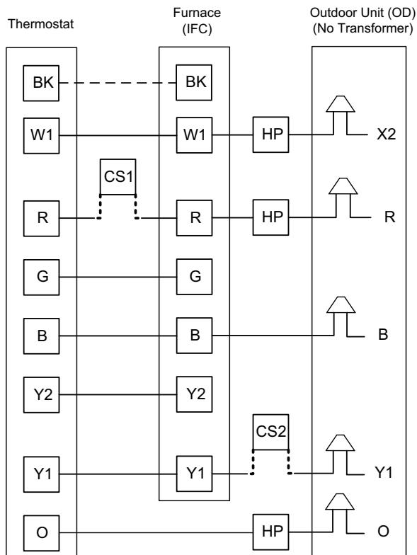
Figure 5. R454-B – link communicating vs heat pump or AC with non communicating L8V1 furnace
