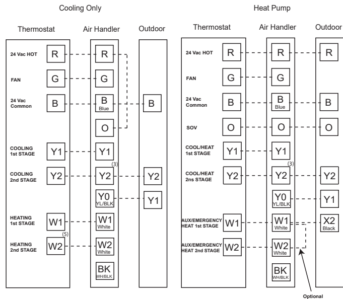
Figure 4. 2-Stage, 2-step
