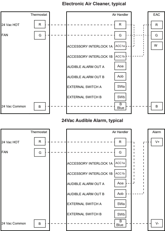
Figure 5. Accessories diagram
