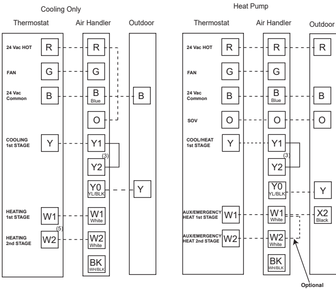
Figure 3. 2-Stage indoor airflow
