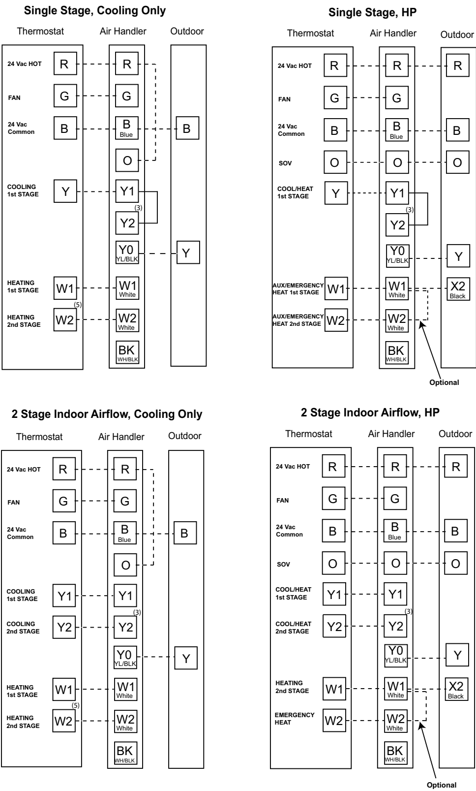
Figure 2. Field wiring diagrams
