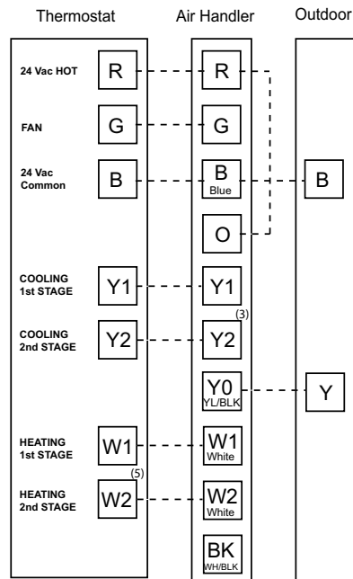
Figure 5. 2 Stage indoor airflow, HP
