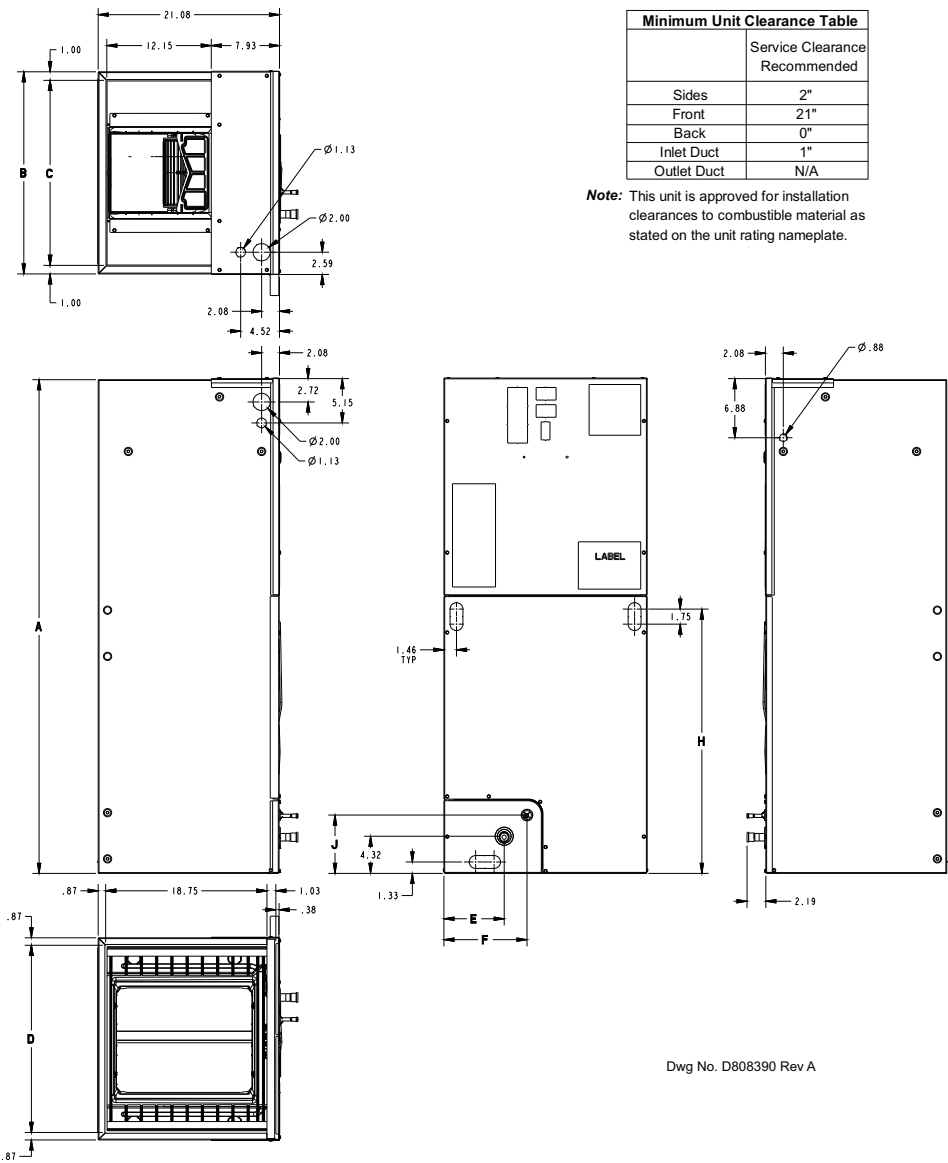
Figure 9. Dimensional data
