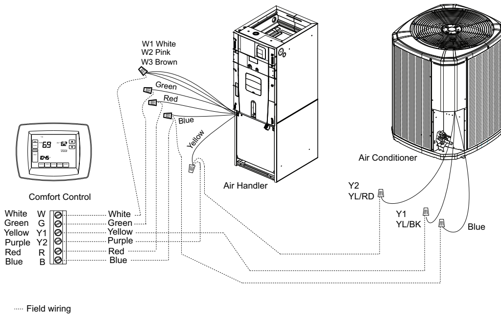
Figure 5. Air handler connection diagram – 2 stage cooling
