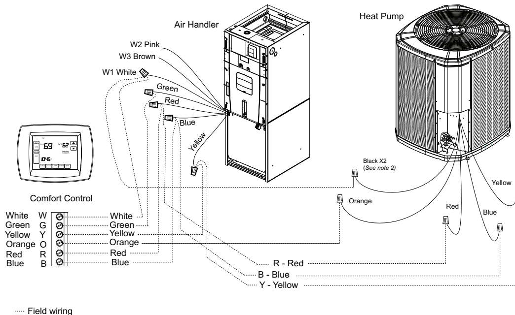
Figure 4. Air handler connection diagram – 1 stage HP
