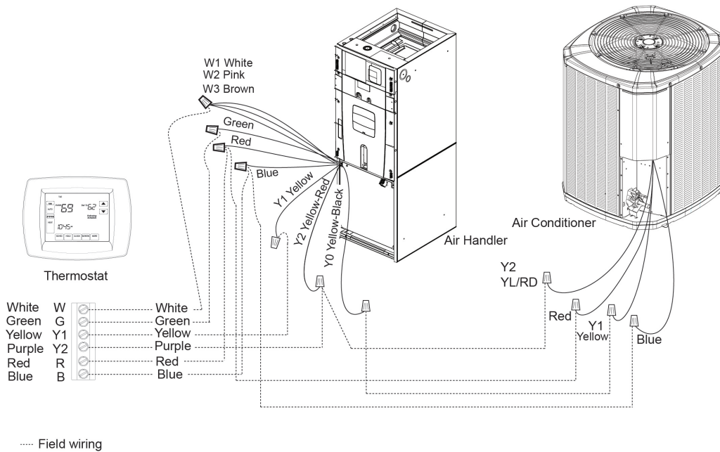
Figure 7. Air handler connection diagram — multi-stage, 24v inverter, cooling only
