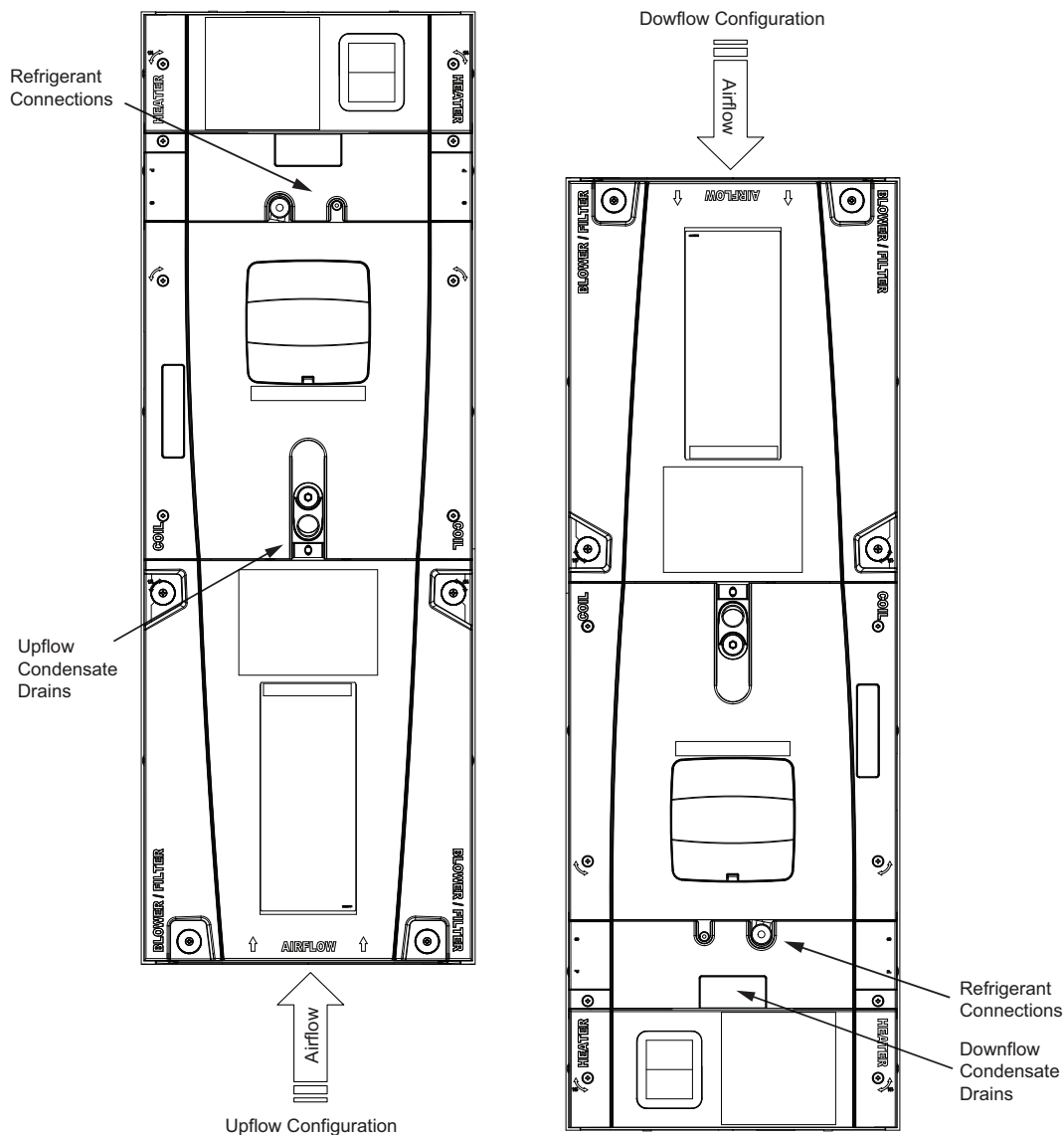
Figure 10. Upflow and downflow configuration
