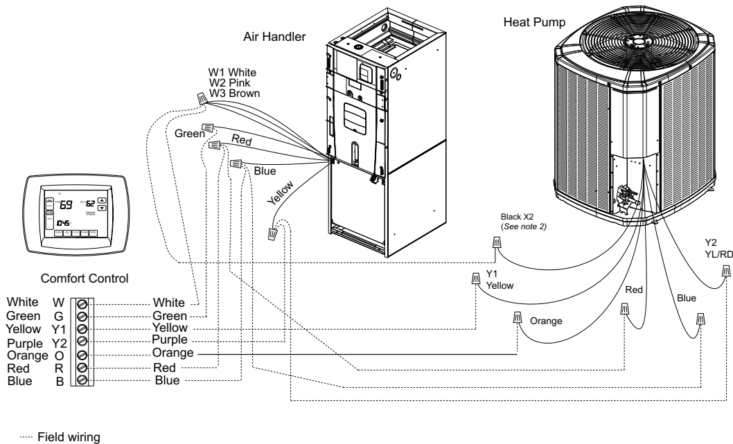
Figure 6. Air handler connection diagram – 2 stage HP
