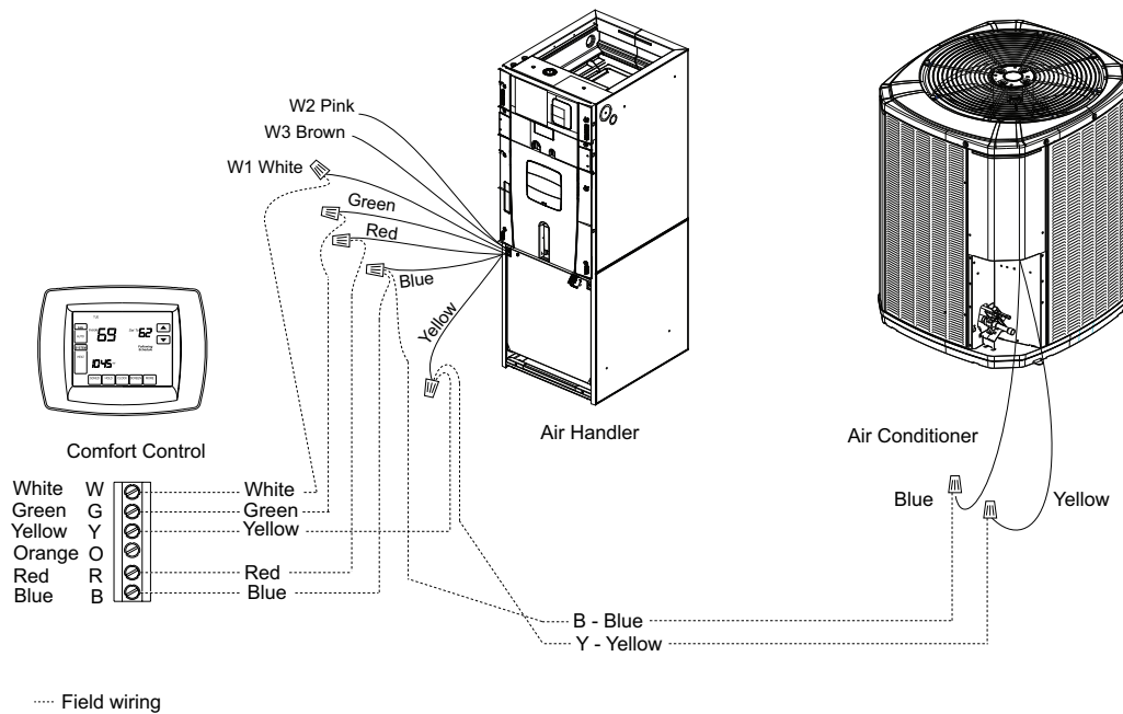
Figure 3. Air handler connection diagram – 1 stage cooling
