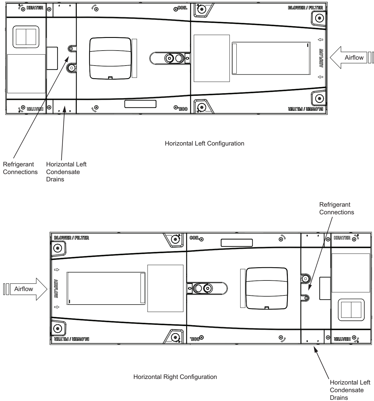
Figure 11. Horizontal left and right configuration
