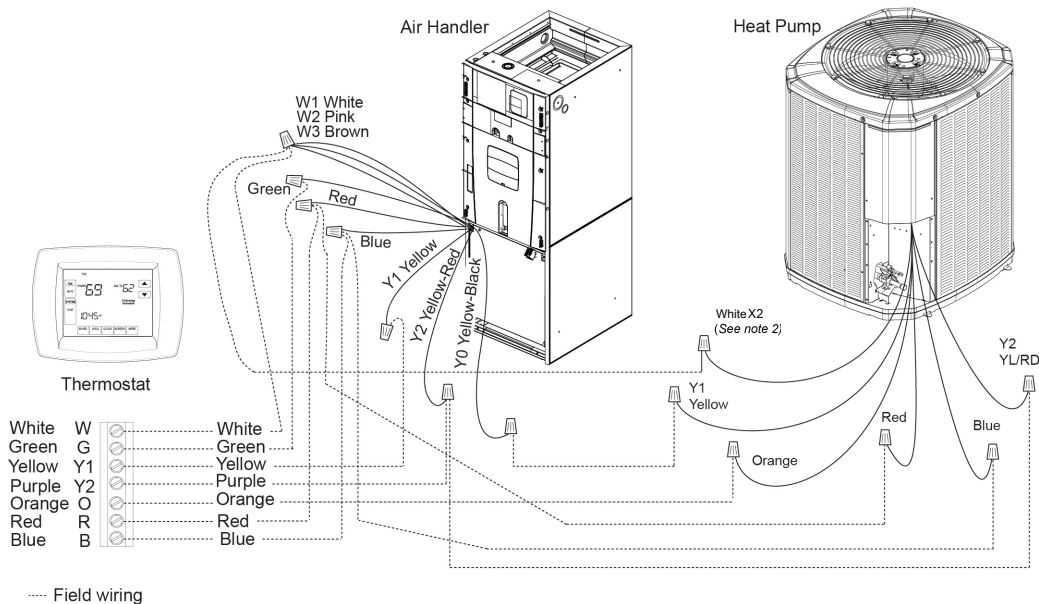
Figure 8. Air handler connection diagram — multi-stage, 24v inverter, HP
