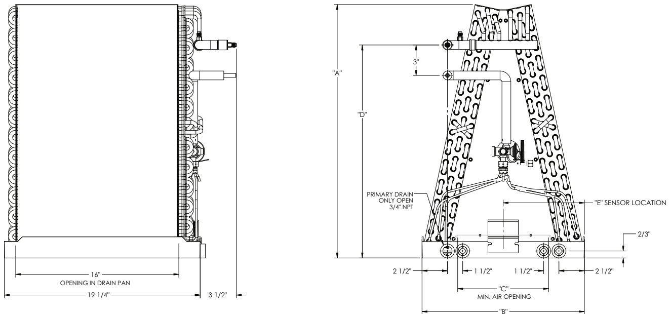
Figure 1. Dimensional drawing
