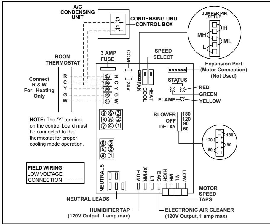
Figure 2. Field Wiring – Low Voltage Connections
