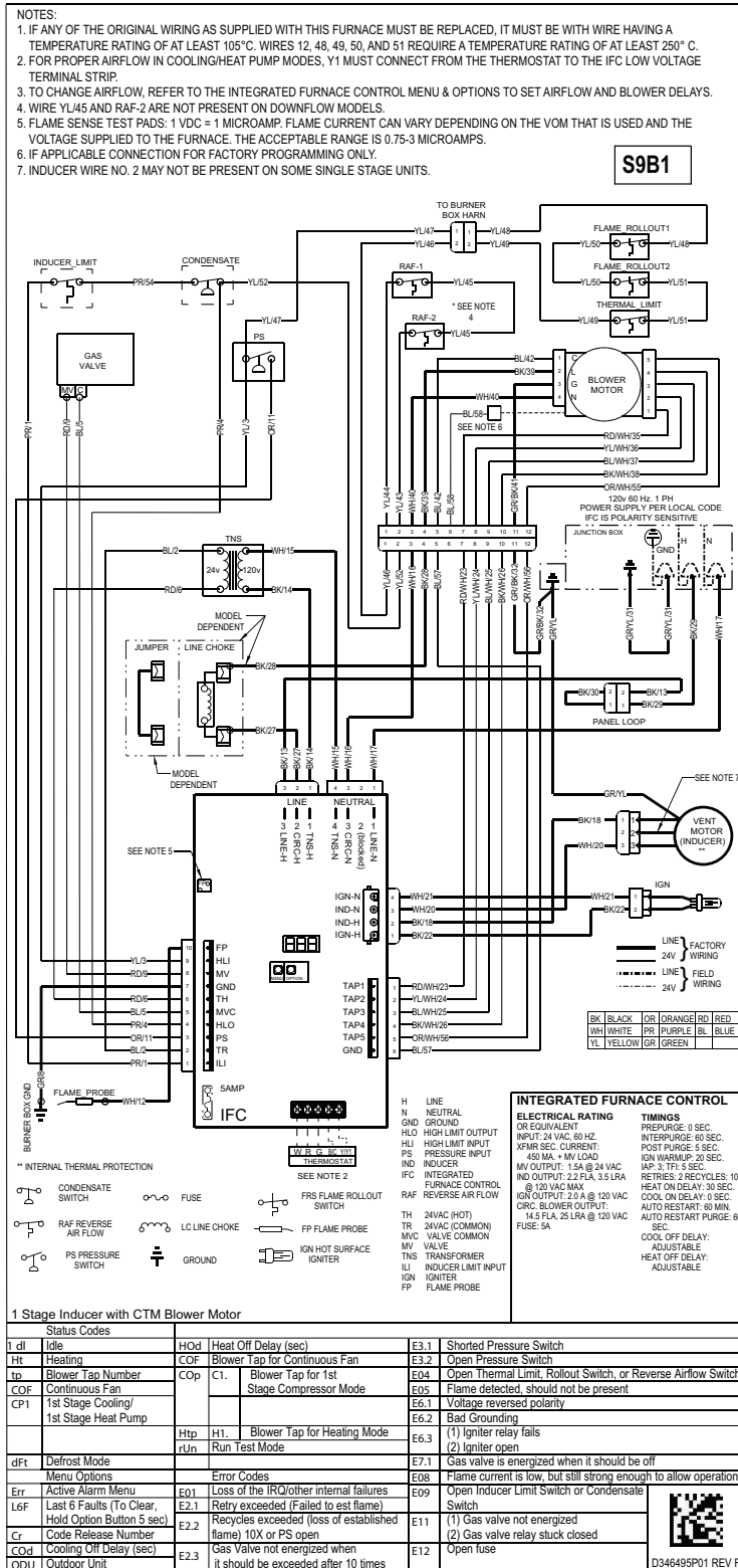
Figure 3. S9B1 Wiring Diagram
