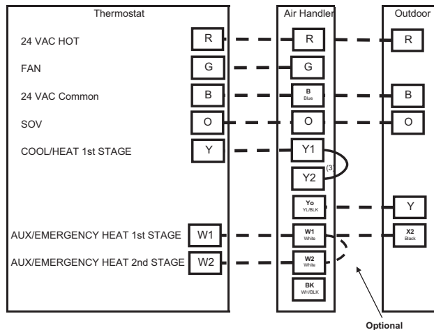
Single Stage, HP, 5TEM6
