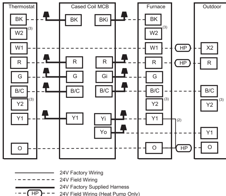
AC or Heat Pump, Typical
