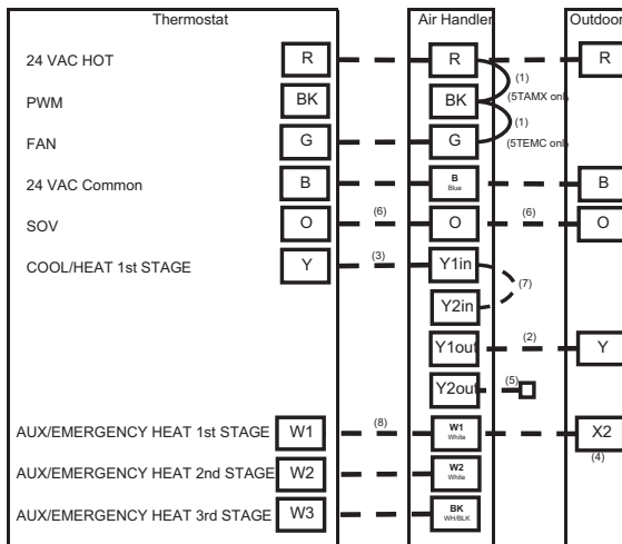
Single Stage, Cooling or Heat Pump, 5TEMC/5TAMX
