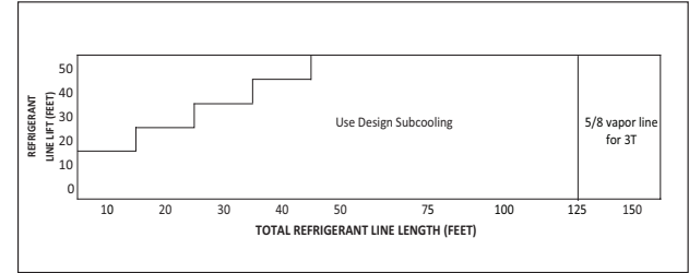
Figure 1. Subcool Charging Corrections – 018A, 024A, 030A, 036A
