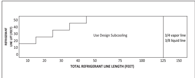
Figure 3. Subcool Charging Corrections – 048A, 060A
