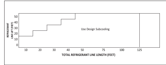
Figure 2. Subcool Charging Corrections – 042A
