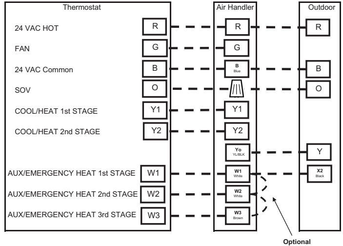
Single Stage, HP, 5TEM4/5TAM5
