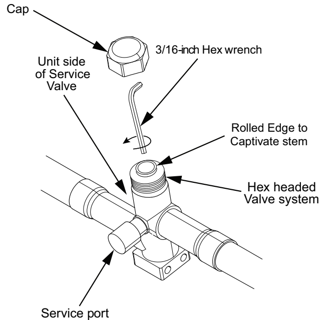
Figure 26. Liquid service valve
