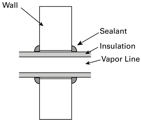
Figure 15. Incorrect lineset installation
