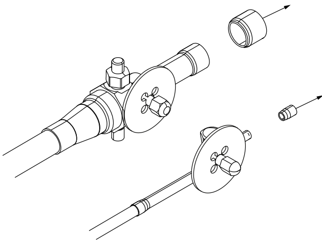
Figure 16. Removal of caps or plugs from pipe ends
