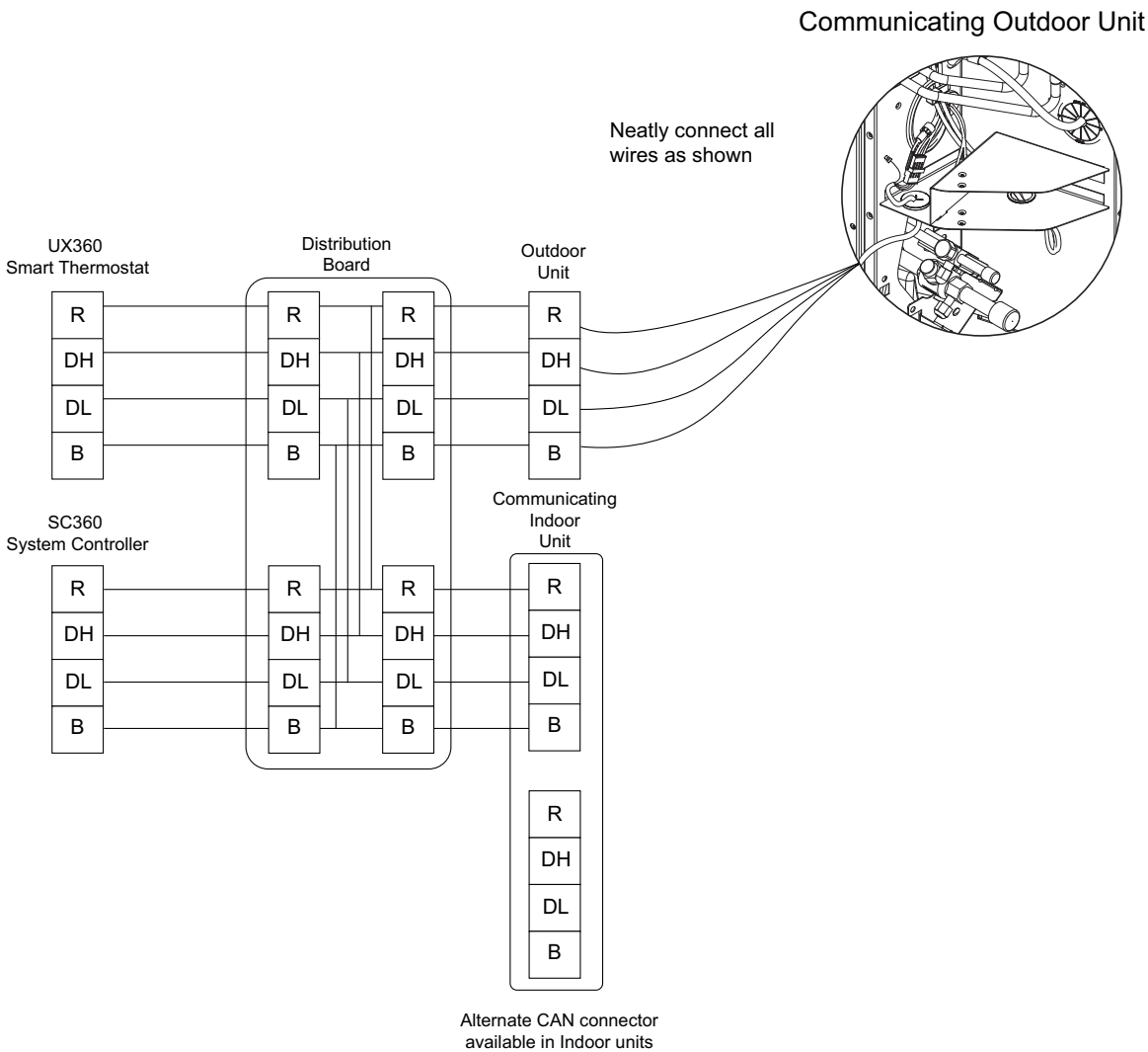
Figure 27. Low-voltage hook-up diagrams in Link mode
