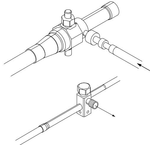
Figure 18. Purging of refrigerant lines
