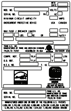
Figure 29. Nameplate location
