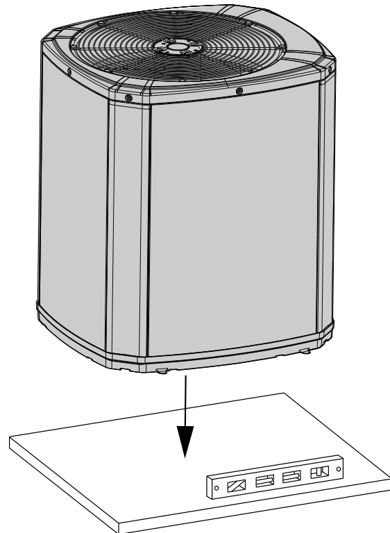
Figure 8. Install the unit on a support pad
