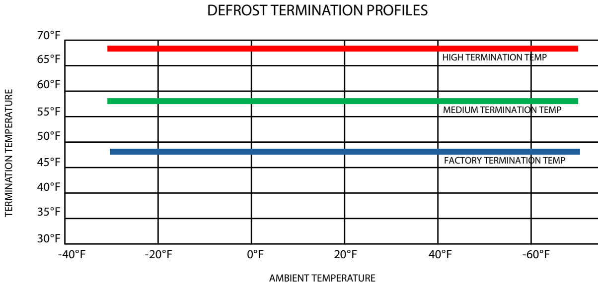
Figure 42. Defrost termination profiles
