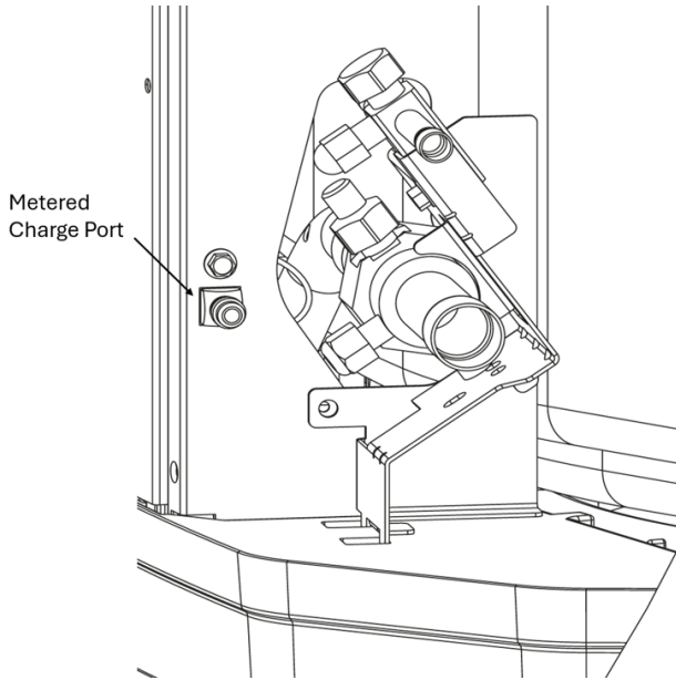
Figure 39. Charge port
