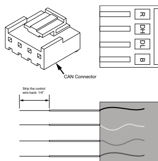
Figure 28. For use with 18 gauge solid core thermostat wire
