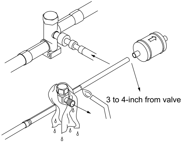
Figure 19. Wrapping of wet rag
