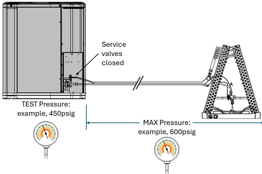
Figure 22. Check for leaks
