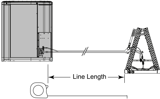
Figure 9. Example of measuring refrigerant line
