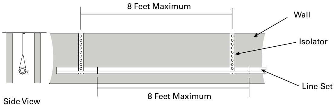
Figure 13. Isolation in wall spaces
