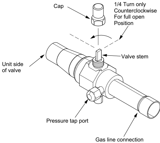
Figure 25. Gas service valve
