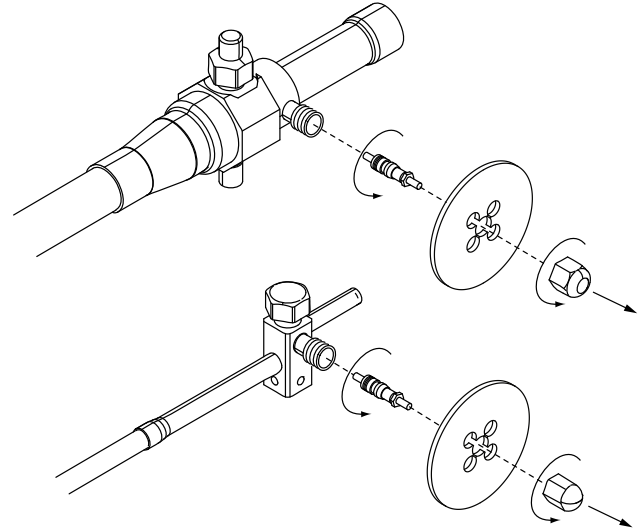
Figure 18. Purging of refrigerant lines
