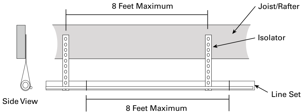
Figure 12. Isolation from a joist/rafter
