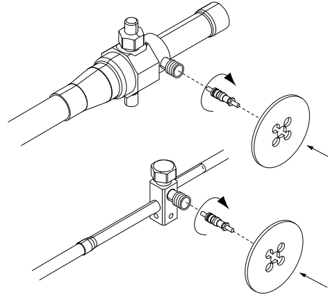
Figure 20. Re-installation of pressure valve cores and plastic tabs
