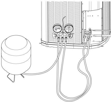
Figure 37. Charging the unit
