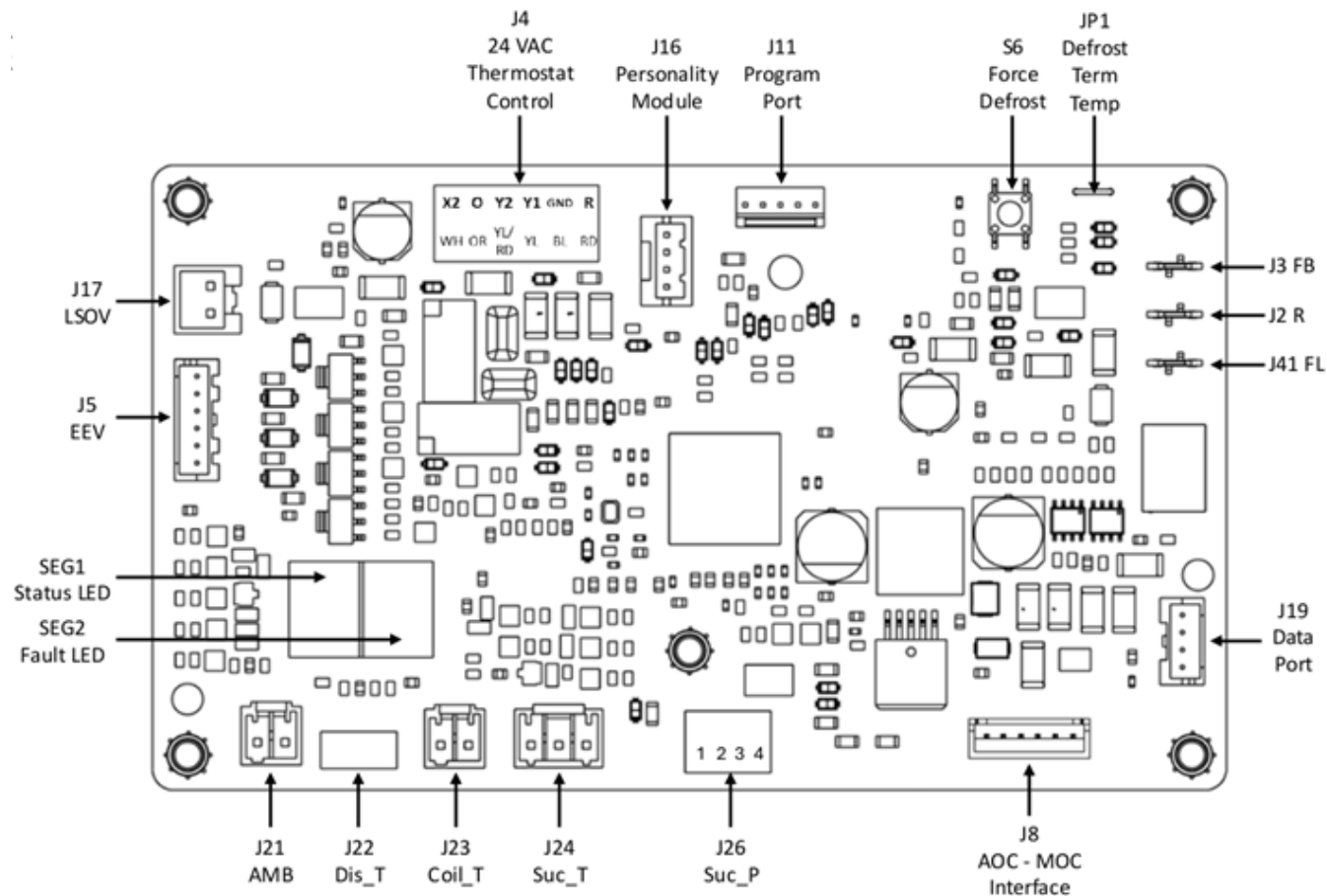
Figure 31. LED indicators
