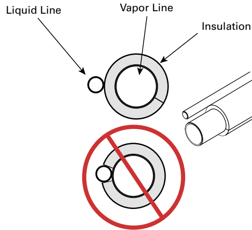
Figure 5. Refrigerant line insulation
