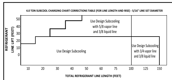
Figure 3. Subcool Charging Corrections – 4.0 Ton
