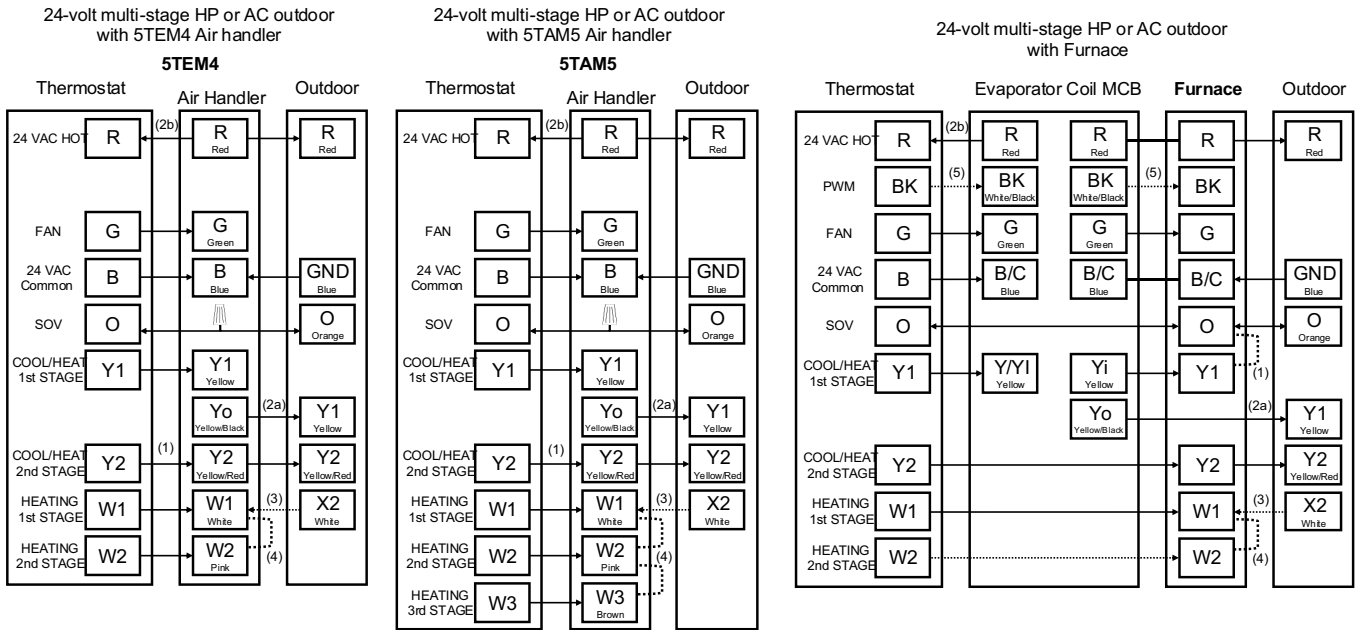
Figure 26. Connection diagrams – 5STEM4, 5TAM5
