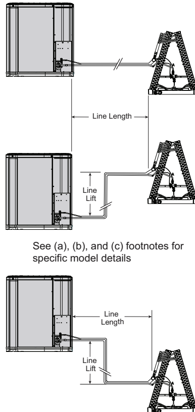
Figure 2. Line length
