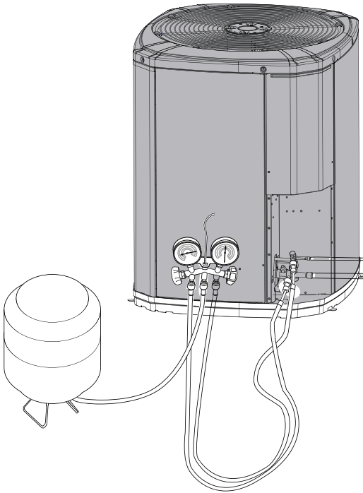
Figure 36. Adjust refrigerant level
